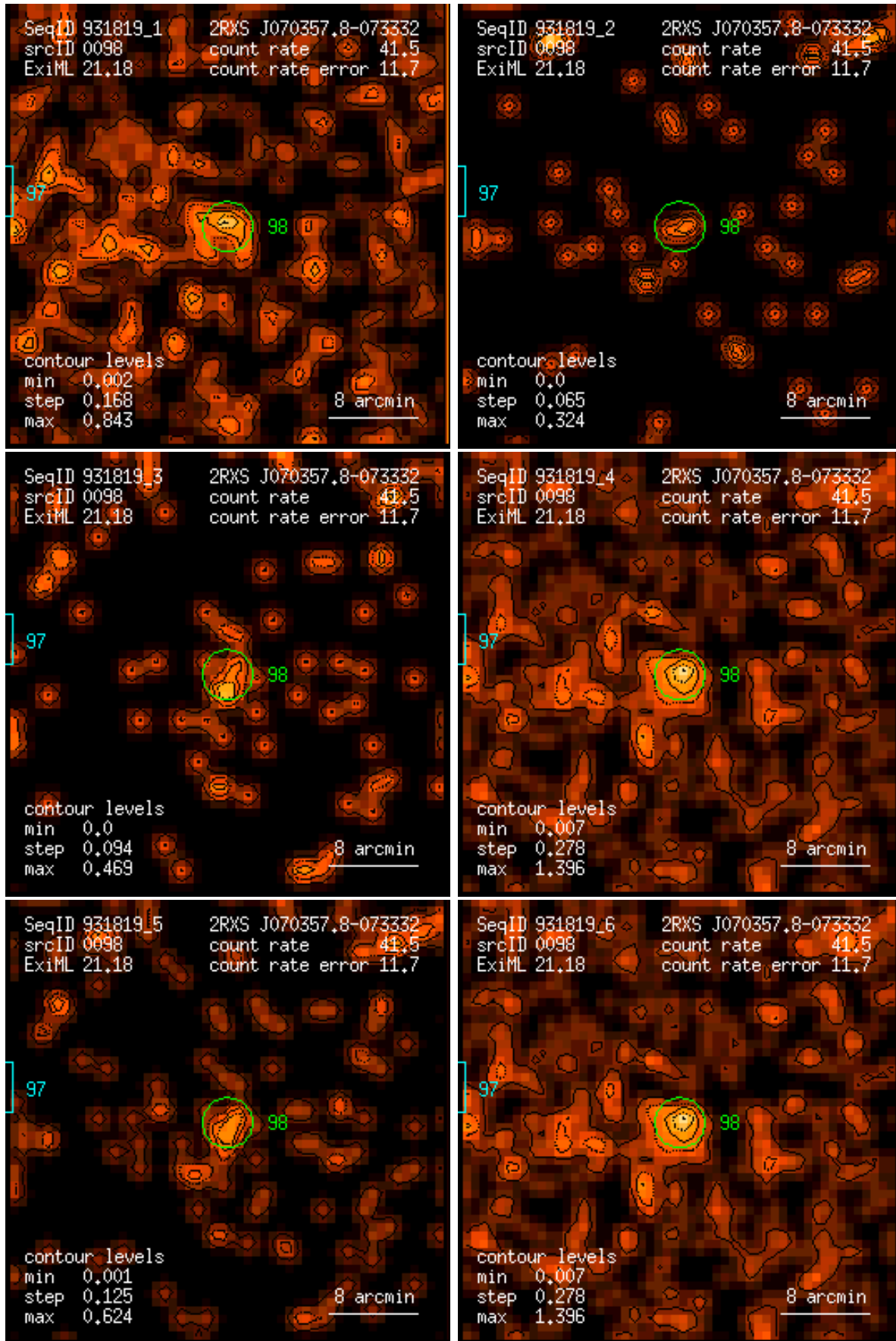
Figure 98: RASS 931819: detection 0098: band rate images, Gaussian filter: (1) PSPC channels 11 – 41, (2) 52 – 90, (3) 91 – 201, (4) 11 – 235, (5) 52 – 201, (6) 11 – 201. Broad band rates in counts/ks. Band rate contour levels in counts/ks/arcmin 2 .
