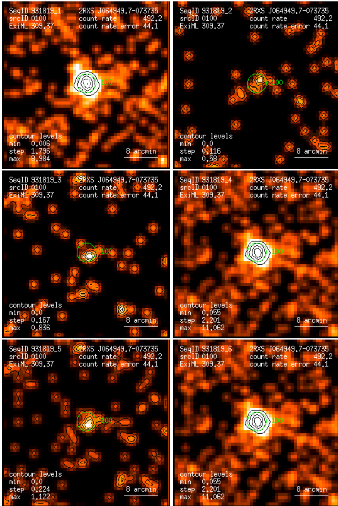
Figure 100: RASS 931819: detection 0100: band rate images, Gaussian filter: (1) PSPC channels 11 – 41, (2) 52 – 90, (3) 91 – 201, (4) 11 – 235, (5) 52 – 201, (6) 11 – 201. Broad band rates in counts/ks. Band rate contour levels in counts/ks/arcmin 2 .
