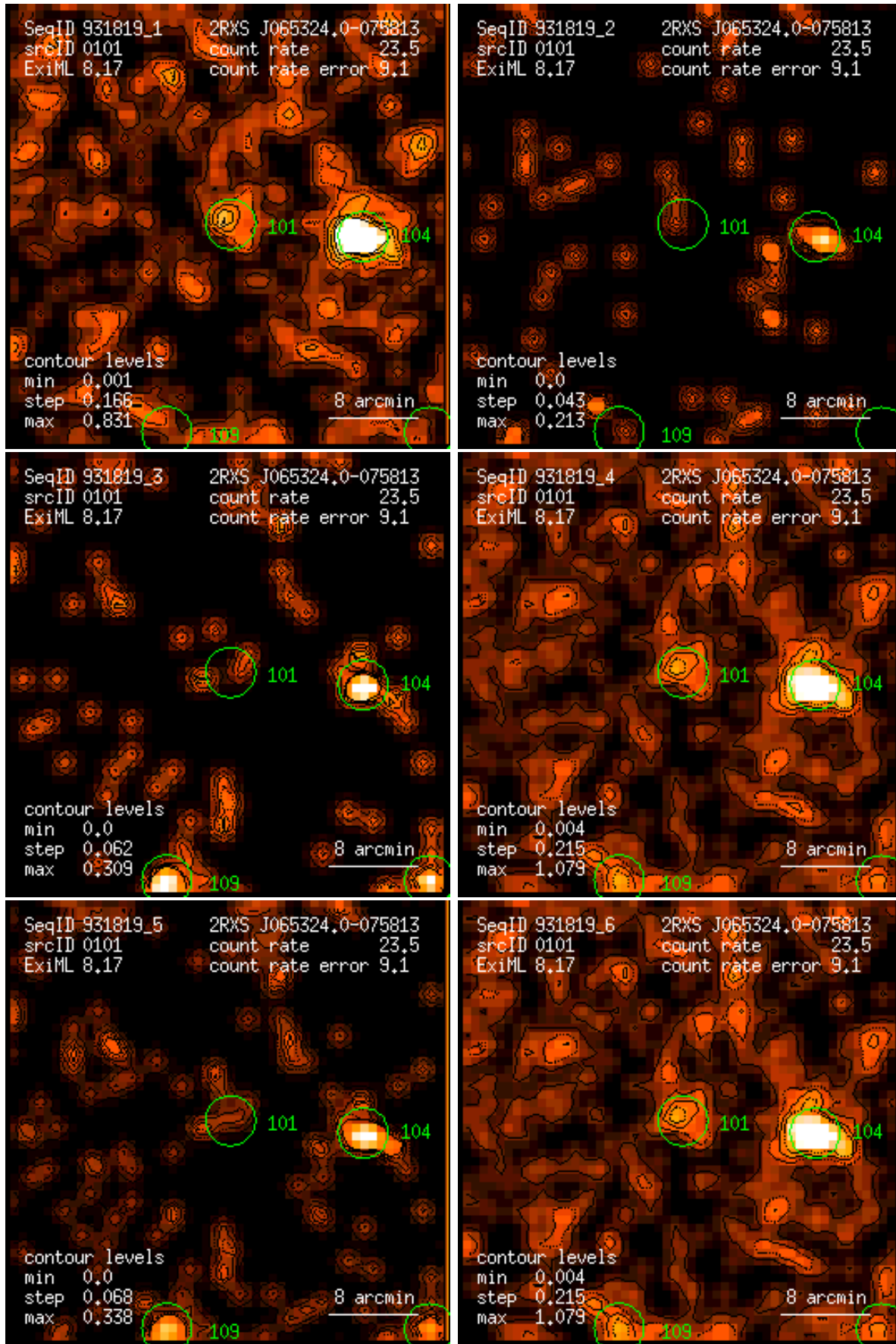
Figure 101: RASS 931819: detection 0101: band rate images, Gaussian filter: (1) PSPC channels 11 – 41, (2) 52 – 90, (3) 91 – 201, (4) 11 – 235, (5) 52 – 201, (6) 11 – 201. Broad band rates in counts/ks. Band rate contour levels in counts/ks/arcmin 2 .
