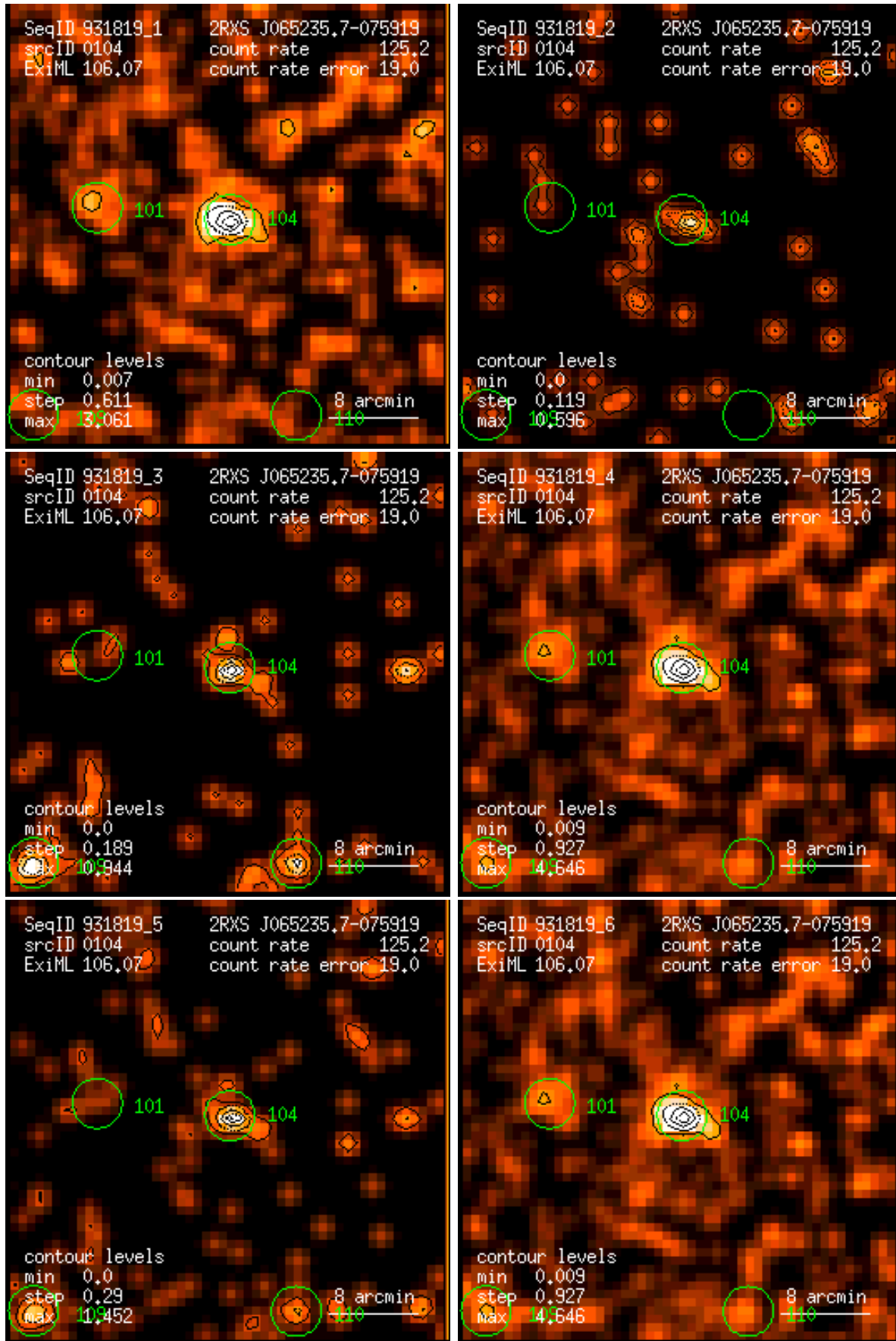
Figure 104: RASS 931819: detection 0104: band rate images, Gaussian filter: (1) PSPC channels 11 – 41, (2) 52 – 90, (3) 91 – 201, (4) 11 – 235, (5) 52 – 201, (6) 11 – 201. Broad band rates in counts/ks. Band rate contour levels in counts/ks/arcmin 2 .
