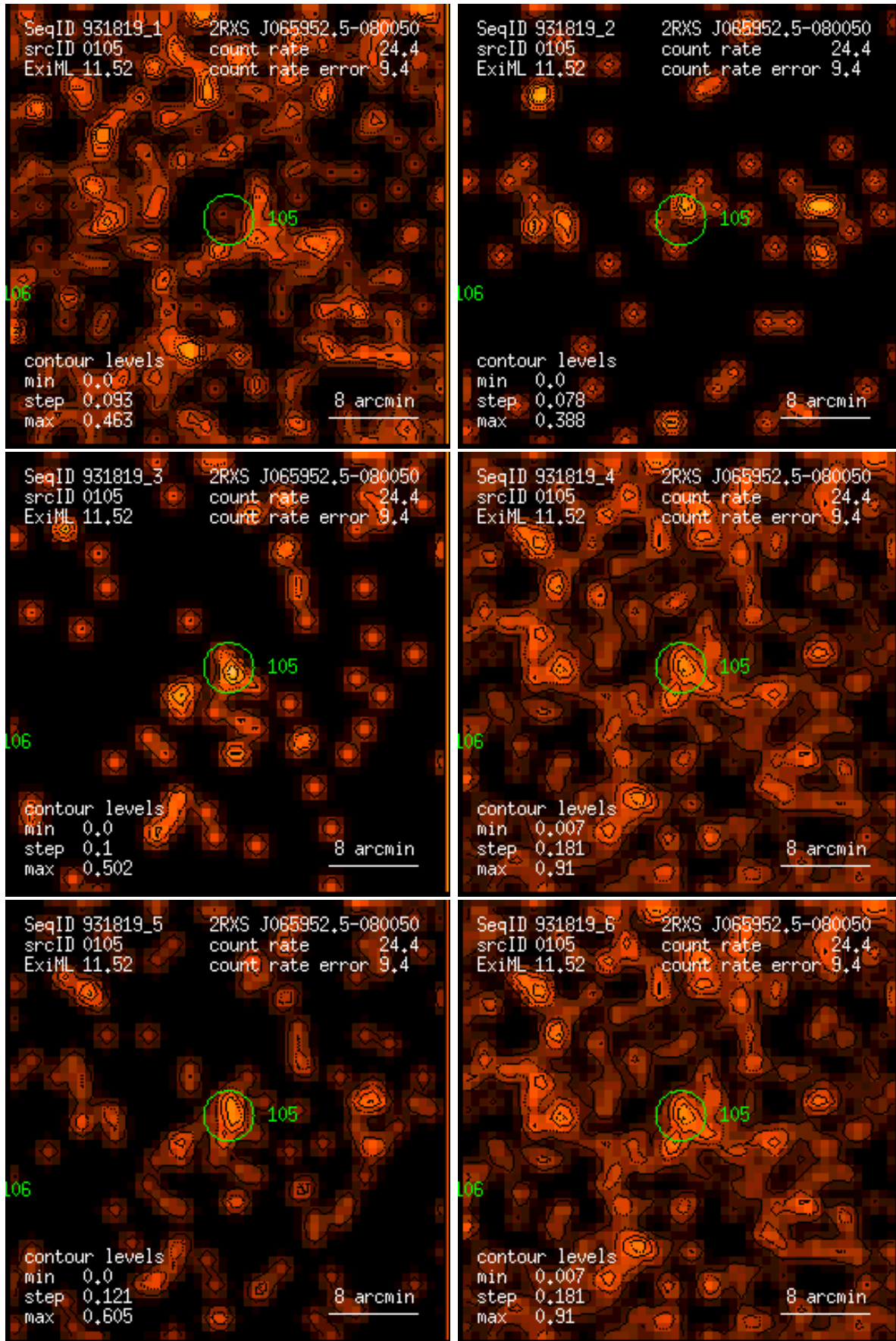
Figure 105: RASS 931819: detection 0105: band rate images, Gaussian filter: (1) PSPC channels 11 – 41, (2) 52 – 90, (3) 91 – 201, (4) 11 – 235, (5) 52 – 201, (6) 11 – 201. Broad band rates in counts/ks. Band rate contour levels in counts/ks/arcmin 2 .
