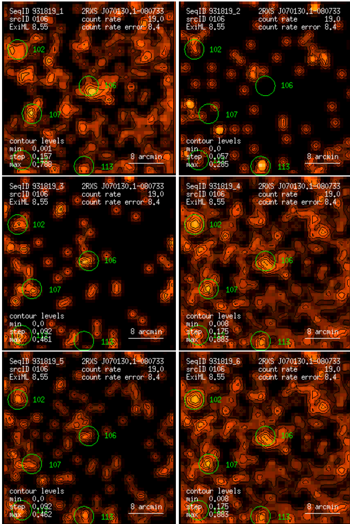
Figure 106: RASS 931819: detection 0106: band rate images, Gaussian filter: (1) PSPC channels 11 – 41, (2) 52 – 90, (3) 91 – 201, (4) 11 – 235, (5) 52 – 201, (6) 11 – 201. Broad band rates in counts/ks. Band rate contour levels in counts/ks/arcmin 2 .
