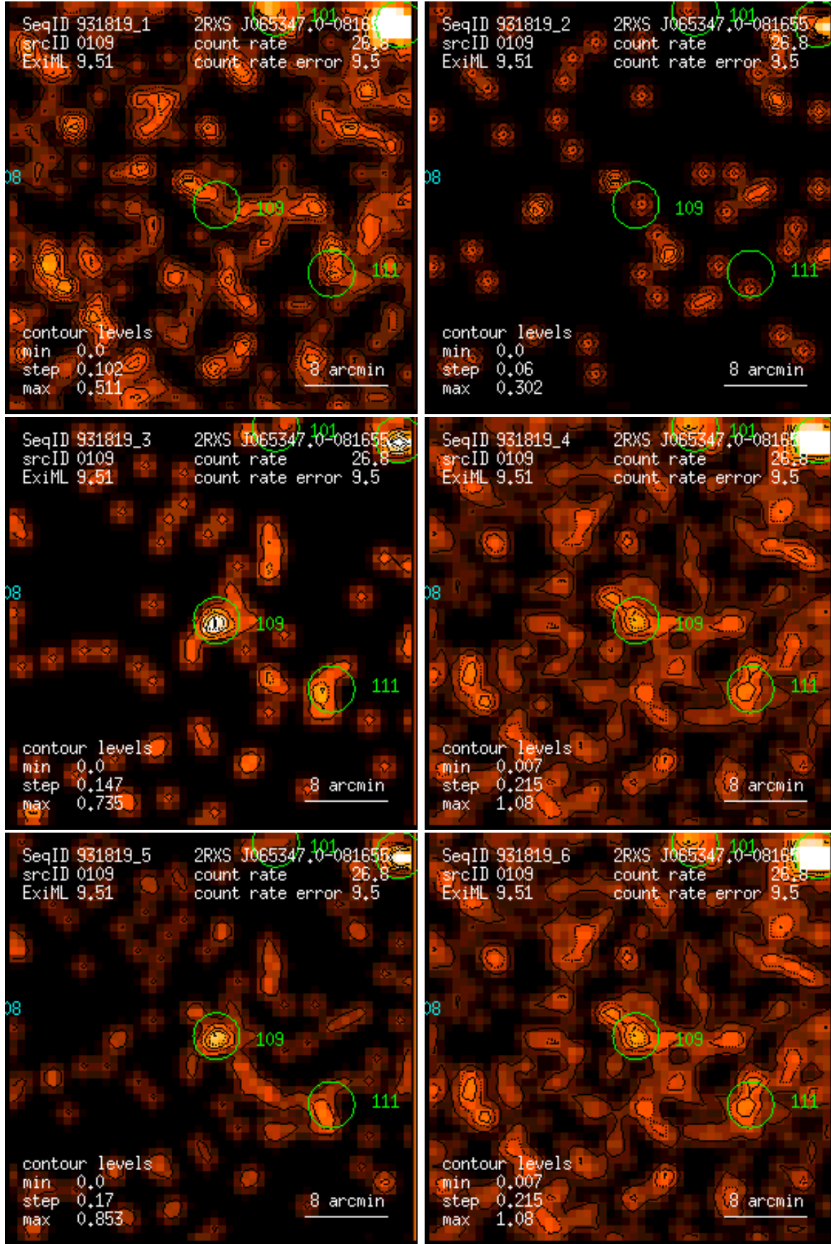
Figure 109: RASS 931819: detection 0109: band rate images, Gaussian filter: (1) PSPC channels 11 – 41, (2) 52 – 90, (3) 91 – 201, (4) 11 – 235, (5) 52 – 201, (6) 11 – 201. Broad band rates in counts/ks. Band rate contour levels in counts/ks/arcmin 2 .
