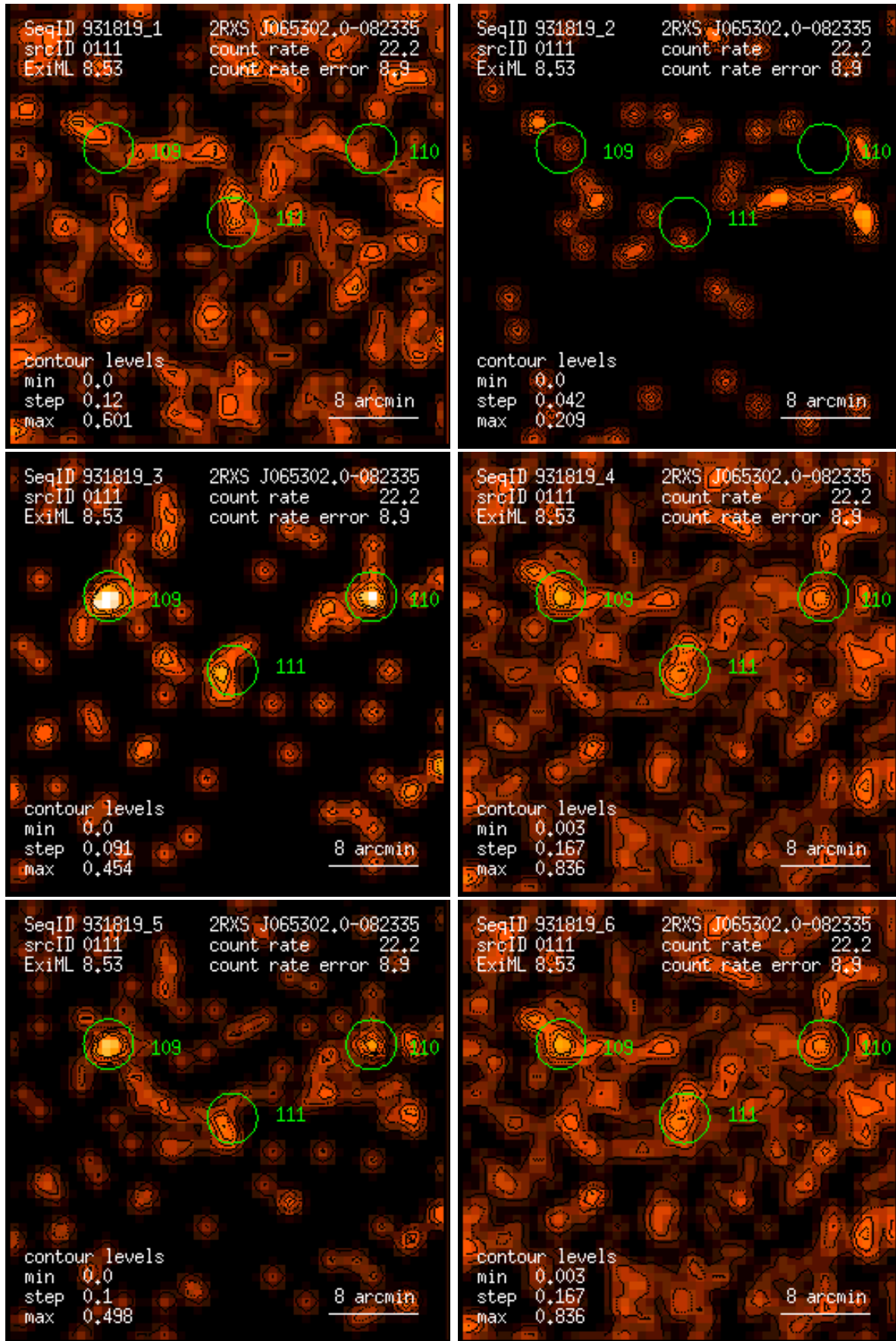
Figure 111: RASS 931819: detection 0111: band rate images, Gaussian filter: (1) PSPC channels 11 – 41, (2) 52 – 90, (3) 91 – 201, (4) 11 – 235, (5) 52 – 201, (6) 11 – 201. Broad band rates in counts/ks. Band rate contour levels in counts/ks/arcmin 2 .
