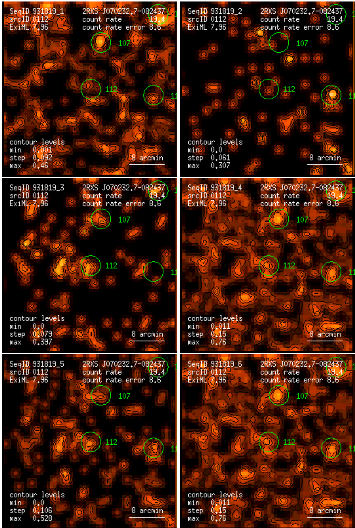
Figure 112: RASS 931819: detection 0112: band rate images, Gaussian filter: (1) PSPC channels 11 – 41, (2) 52 – 90, (3) 91 – 201, (4) 11 – 235, (5) 52 – 201, (6) 11 – 201. Broad band rates in counts/ks. Band rate contour levels in counts/ks/arcmin 2 .
