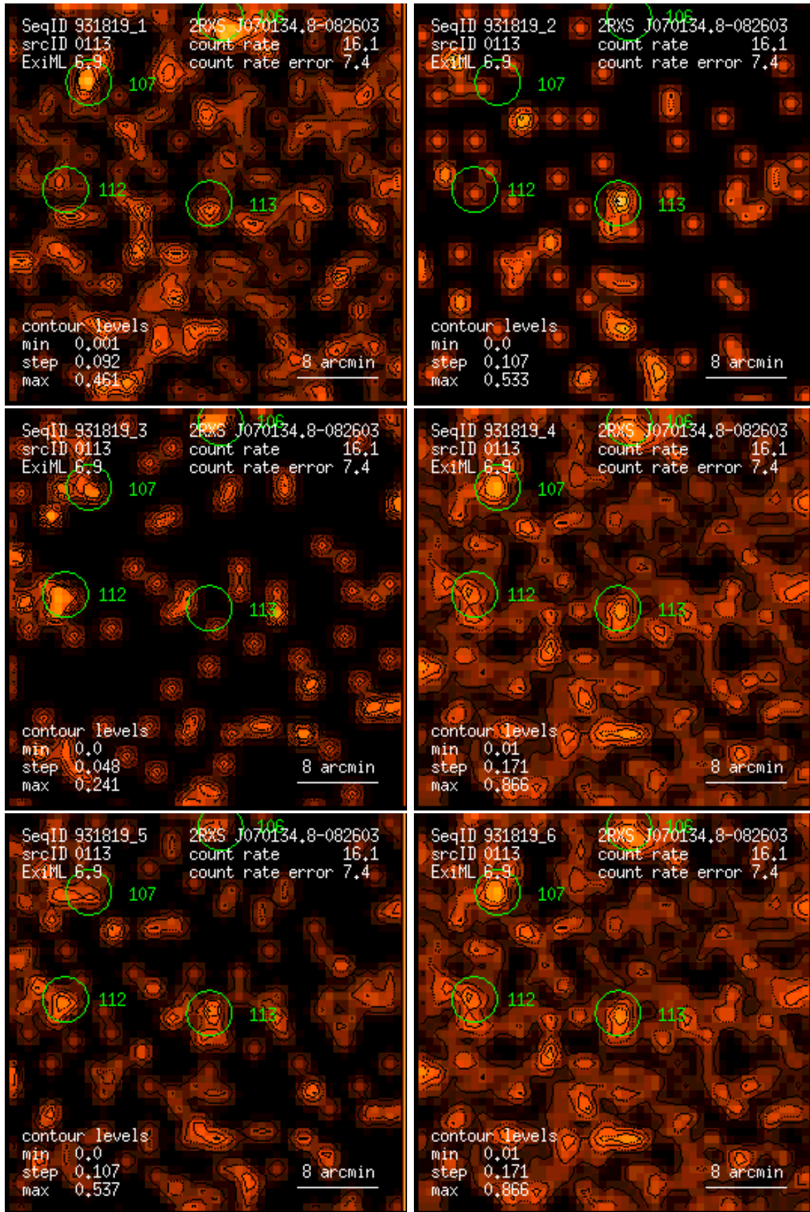
Figure 113: RASS 931819: detection 0113: band rate images, Gaussian filter: (1) PSPC channels 11 – 41, (2) 52 – 90, (3) 91 – 201, (4) 11 – 235, (5) 52 – 201, (6) 11 – 201. Broad band rates in counts/ks. Band rate contour levels in counts/ks/arcmin 2 .
