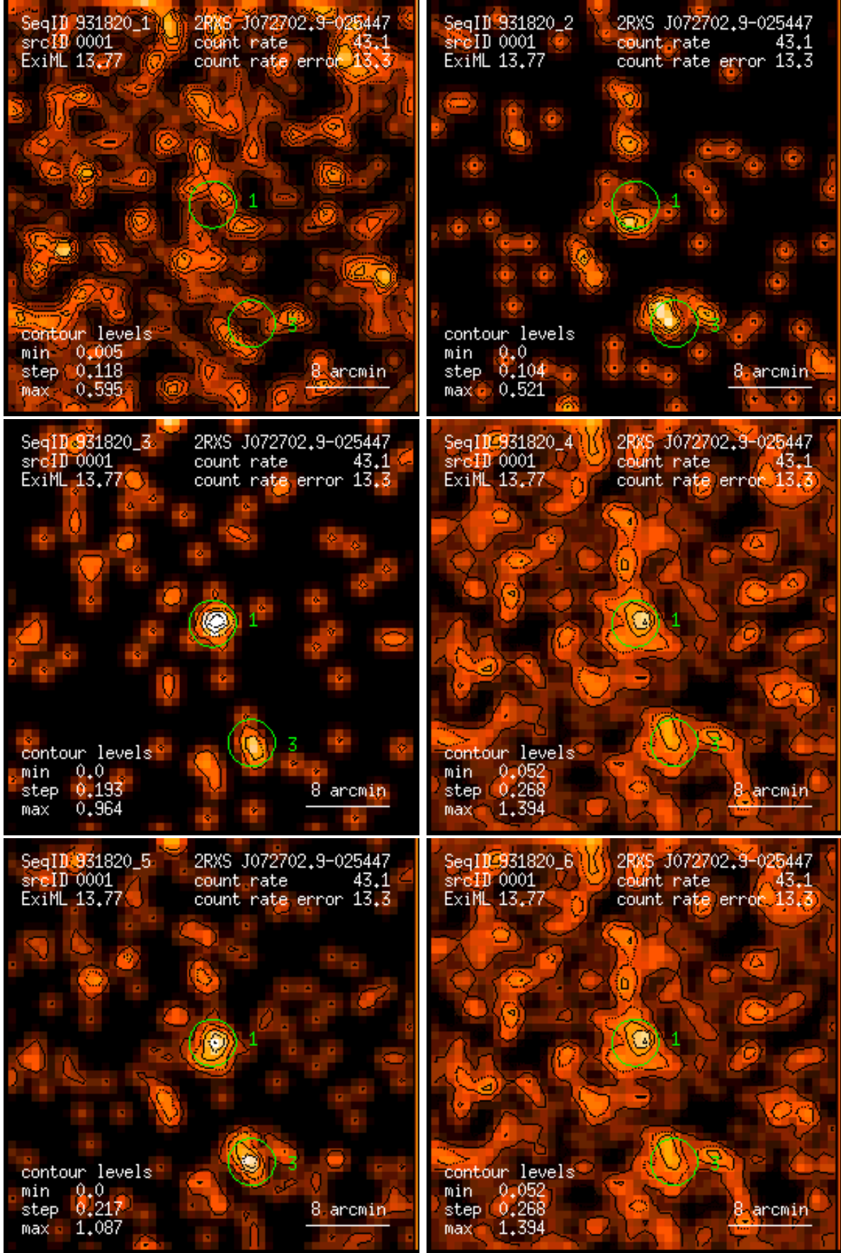
Figure 1: RASS 931820: detection 0001: band rate images, Gaussian filter: (1) PSPC channels 11 – 41, (2) 52 – 90, (3) 91 – 201, (4) 11 – 235, (5) 52 – 201, (6) 11 – 201. Broad band rates in counts/ks. Band rate contour levels in counts/ks/arcmin 2 .
