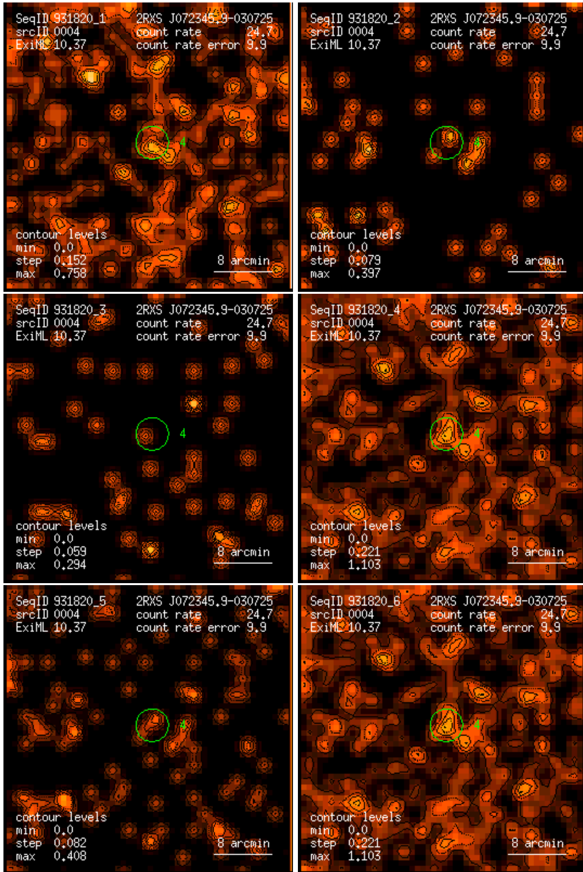
Figure 4: RASS 931820: detection 0004: band rate images, Gaussian filter: (1) PSPC channels 11 – 41, (2) 52 – 90, (3) 91 – 201, (4) 11 – 235, (5) 52 – 201, (6) 11 – 201. Broad band rates in counts/ks. Band rate contour levels in counts/ks/arcmin 2 .
