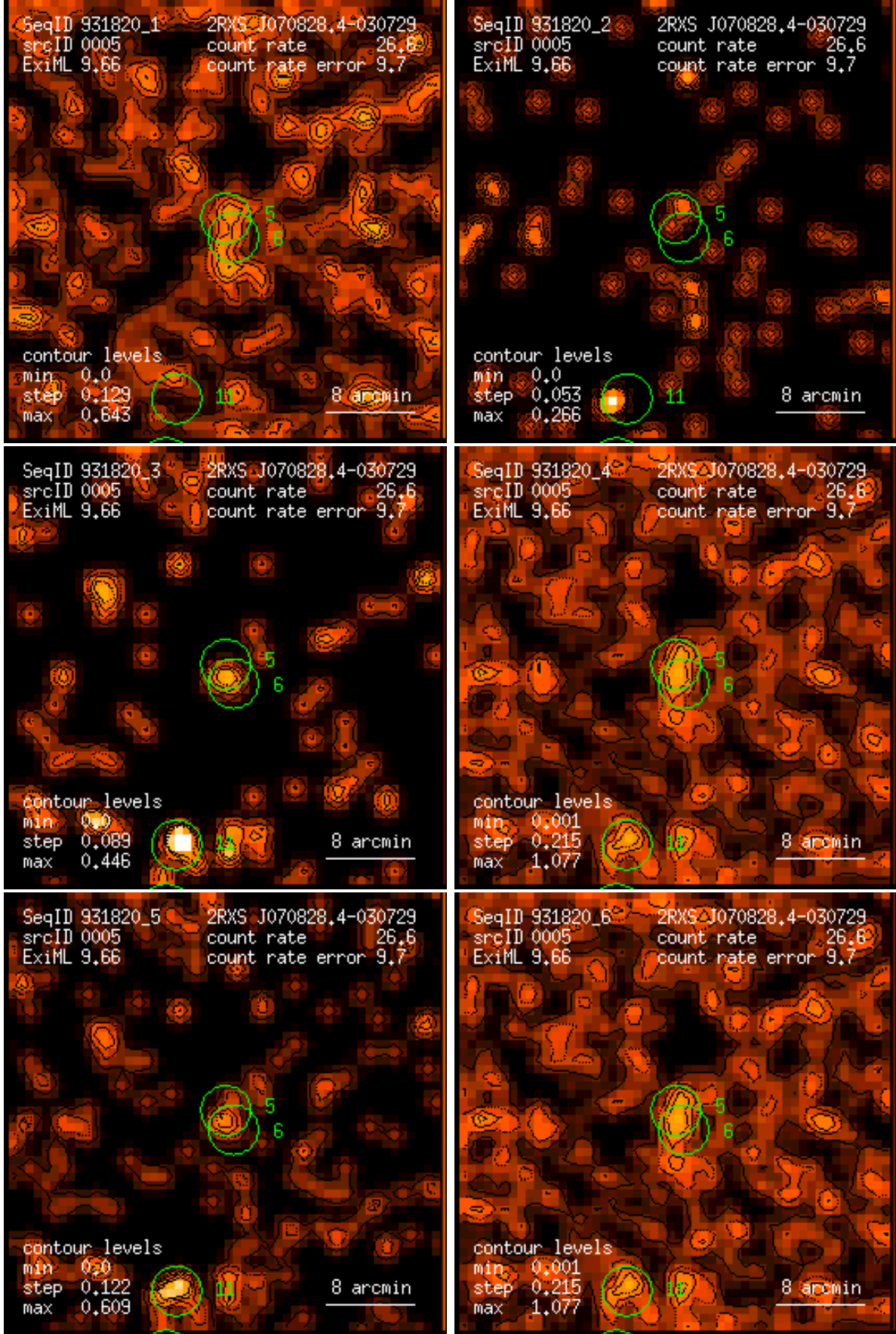
Figure 5: RASS 931820: detection 0005: band rate images, Gaussian filter: (1) PSPC channels 11 – 41, (2) 52 – 90, (3) 91 – 201, (4) 11 – 235, (5) 52 – 201, (6) 11 – 201. Broad band rates in counts/ks. Band rate contour levels in counts/ks/arcmin 2 .
