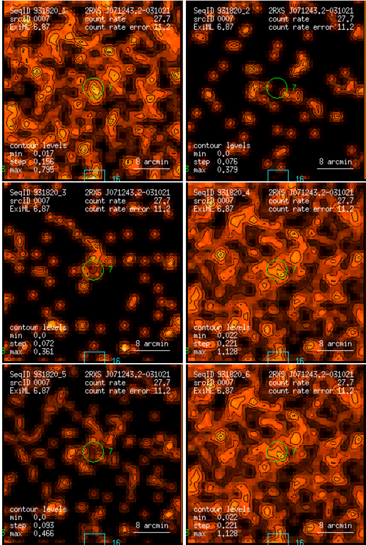
Figure 7: RASS 931820: detection 0007: band rate images, Gaussian filter: (1) PSPC channels 11 – 41, (2) 52 – 90, (3) 91 – 201, (4) 11 – 235, (5) 52 – 201, (6) 11 – 201. Broad band rates in counts/ks. Band rate contour levels in counts/ks/arcmin 2 .
