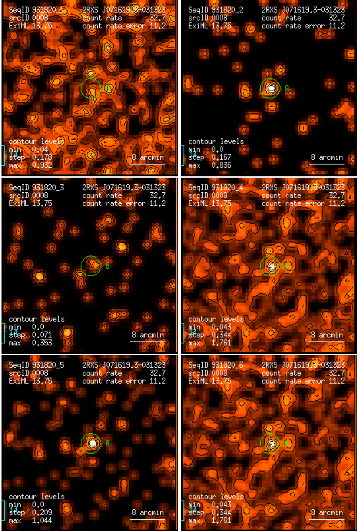
Figure 8: RASS 931820: detection 0008: band rate images, Gaussian filter: (1) PSPC channels 11 – 41, (2) 52 – 90, (3) 91 – 201, (4) 11 – 235, (5) 52 – 201, (6) 11 – 201. Broad band rates in counts/ks. Band rate contour levels in counts/ks/arcmin 2 .
