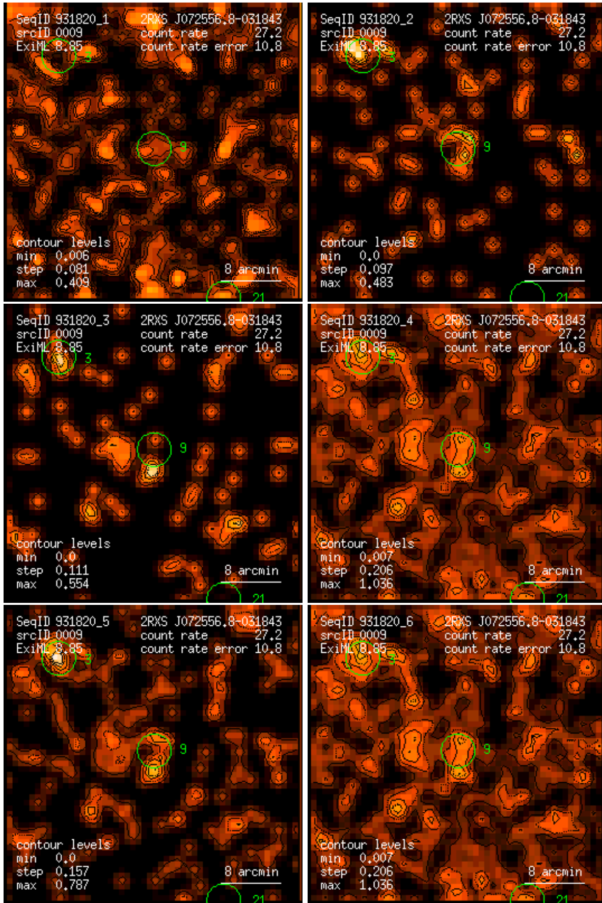
Figure 9: RASS 931820: detection 0009: band rate images, Gaussian filter: (1) PSPC channels 11 – 41, (2) 52 – 90, (3) 91 – 201, (4) 11 – 235, (5) 52 – 201, (6) 11 – 201. Broad band rates in counts/ks. Band rate contour levels in counts/ks/arcmin 2 .
