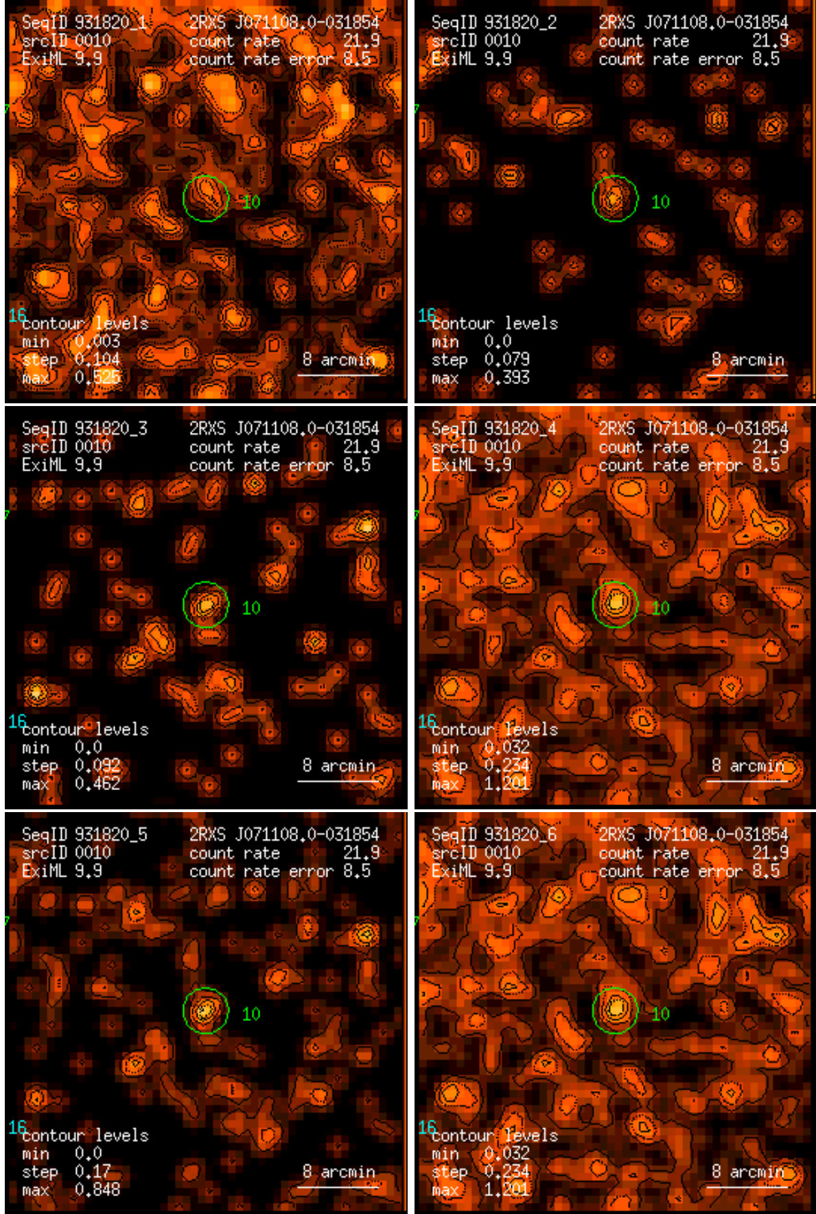
Figure 10: RASS 931820: detection 0010: band rate images, Gaussian filter: (1) PSPC channels 11 – 41, (2) 52 – 90, (3) 91 – 201, (4) 11 – 235, (5) 52 – 201, (6) 11 – 201. Broad band rates in counts/ks. Band rate contour levels in counts/ks/arcmin 2 .
