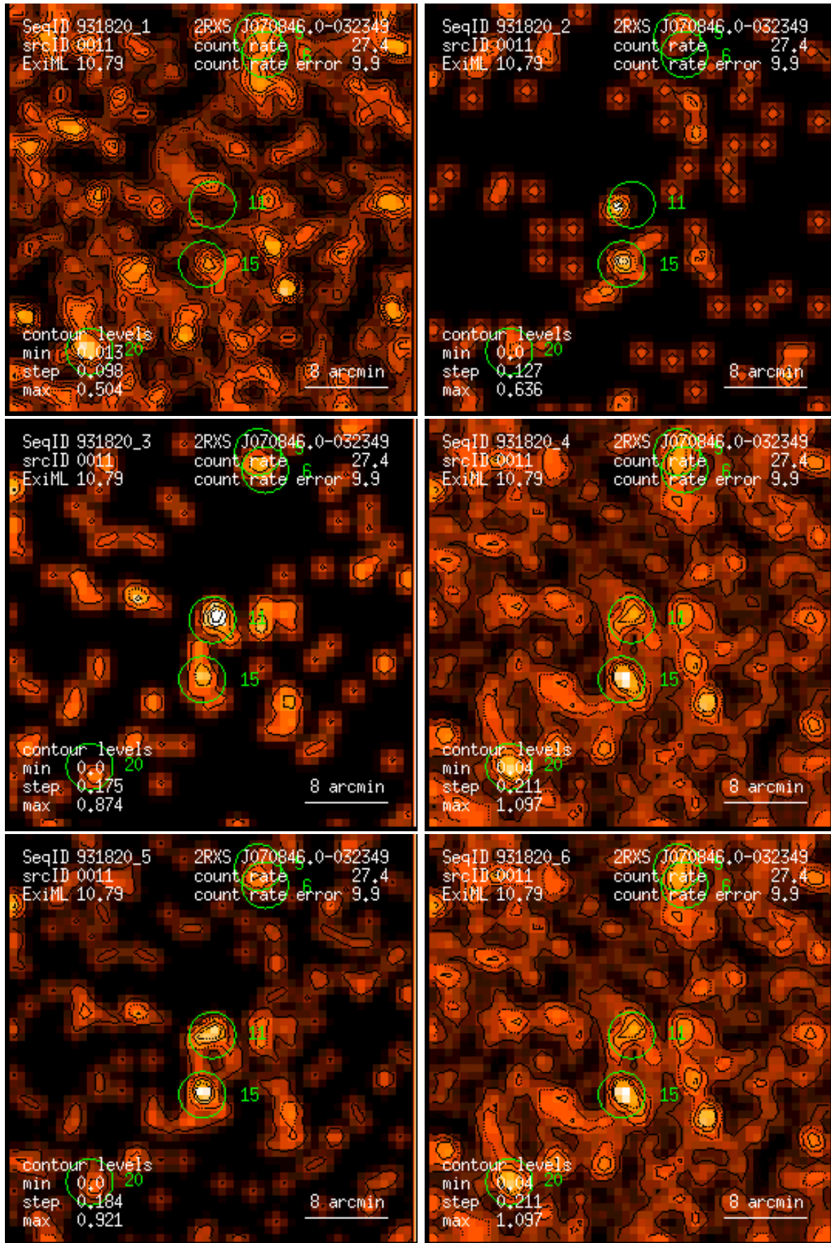
Figure 11: RASS 931820: detection 0011: band rate images, Gaussian filter: (1) PSPC channels 11 – 41, (2) 52 – 90, (3) 91 – 201, (4) 11 – 235, (5) 52 – 201, (6) 11 – 201. Broad band rates in counts/ks. Band rate contour levels in counts/ks/arcmin 2 .
