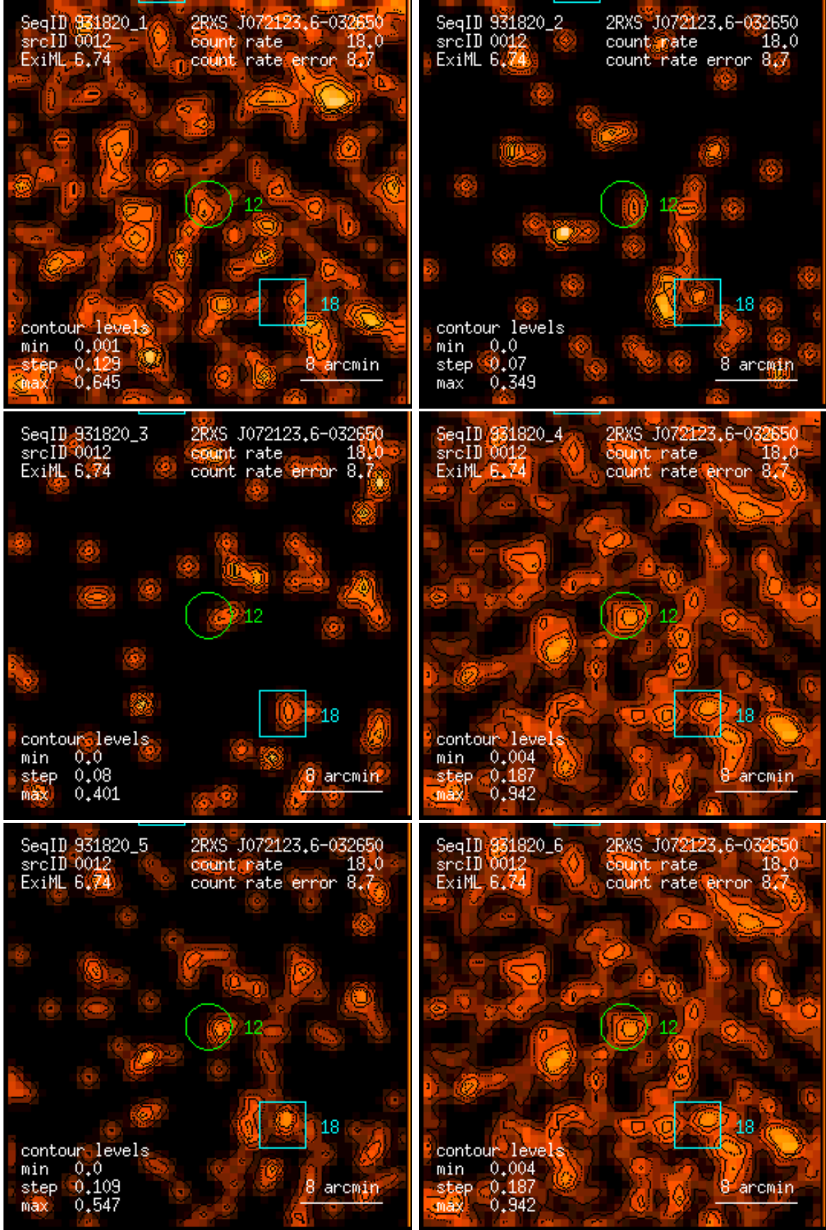
Figure 12: RASS 931820: detection 0012: band rate images, Gaussian filter: (1) PSPC channels 11 – 41, (2) 52 – 90, (3) 91 – 201, (4) 11 – 235, (5) 52 – 201, (6) 11 – 201. Broad band rates in counts/ks. Band rate contour levels in counts/ks/arcmin 2 .
