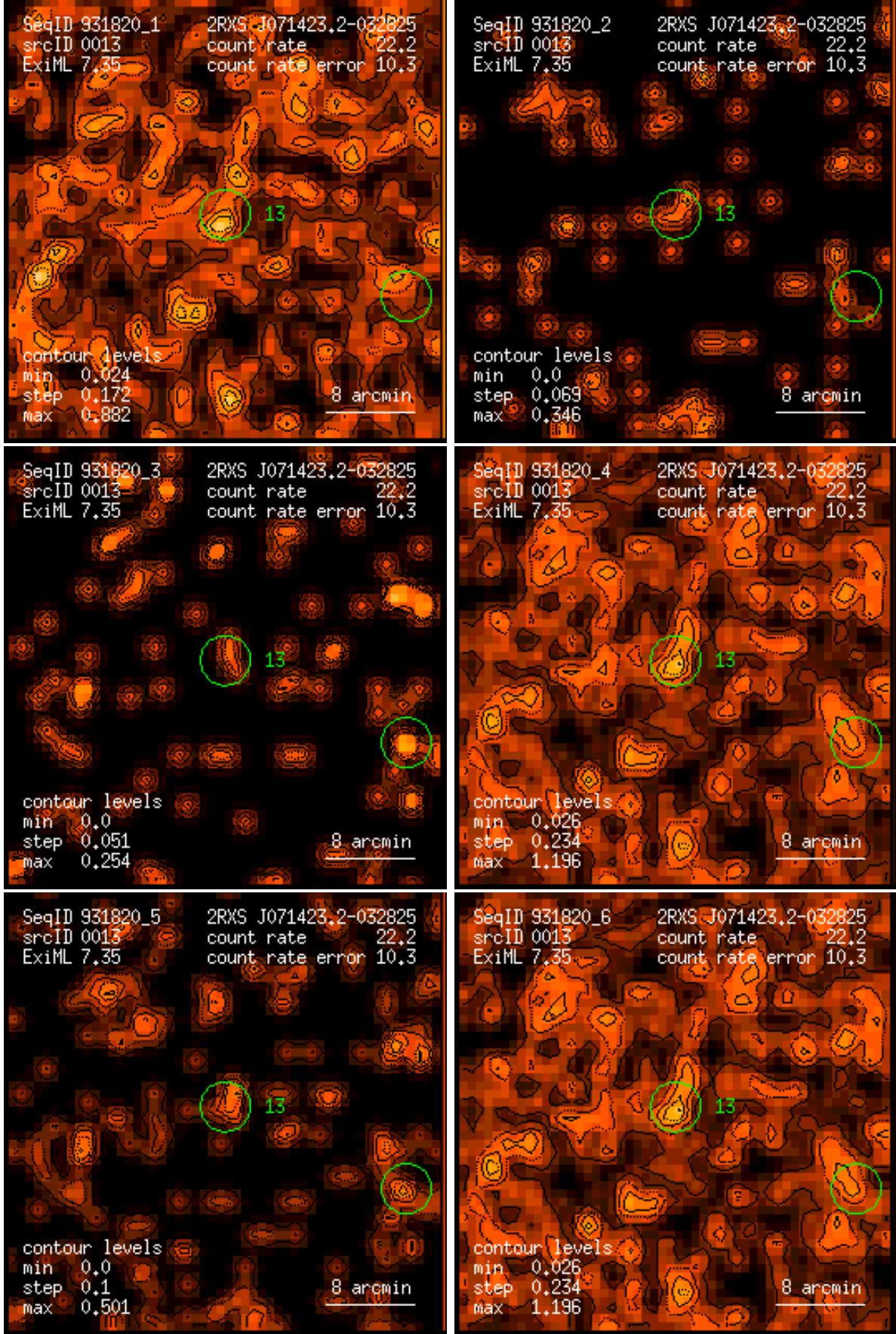
Figure 13: RASS 931820: detection 0013: band rate images, Gaussian filter: (1) PSPC channels 11 – 41, (2) 52 – 90, (3) 91 – 201, (4) 11 – 235, (5) 52 – 201, (6) 11 – 201. Broad band rates in counts/ks. Band rate contour levels in counts/ks/arcmin 2 .
