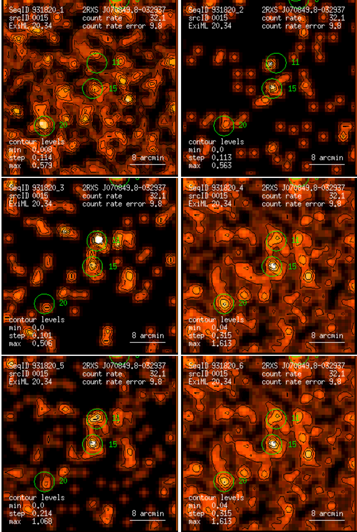
Figure 15: RASS 931820: detection 0015: band rate images, Gaussian filter: (1) PSPC channels 11 – 41, (2) 52 – 90, (3) 91 – 201, (4) 11 – 235, (5) 52 – 201, (6) 11 – 201. Broad band rates in counts/ks. Band rate contour levels in counts/ks/arcmin 2 .
