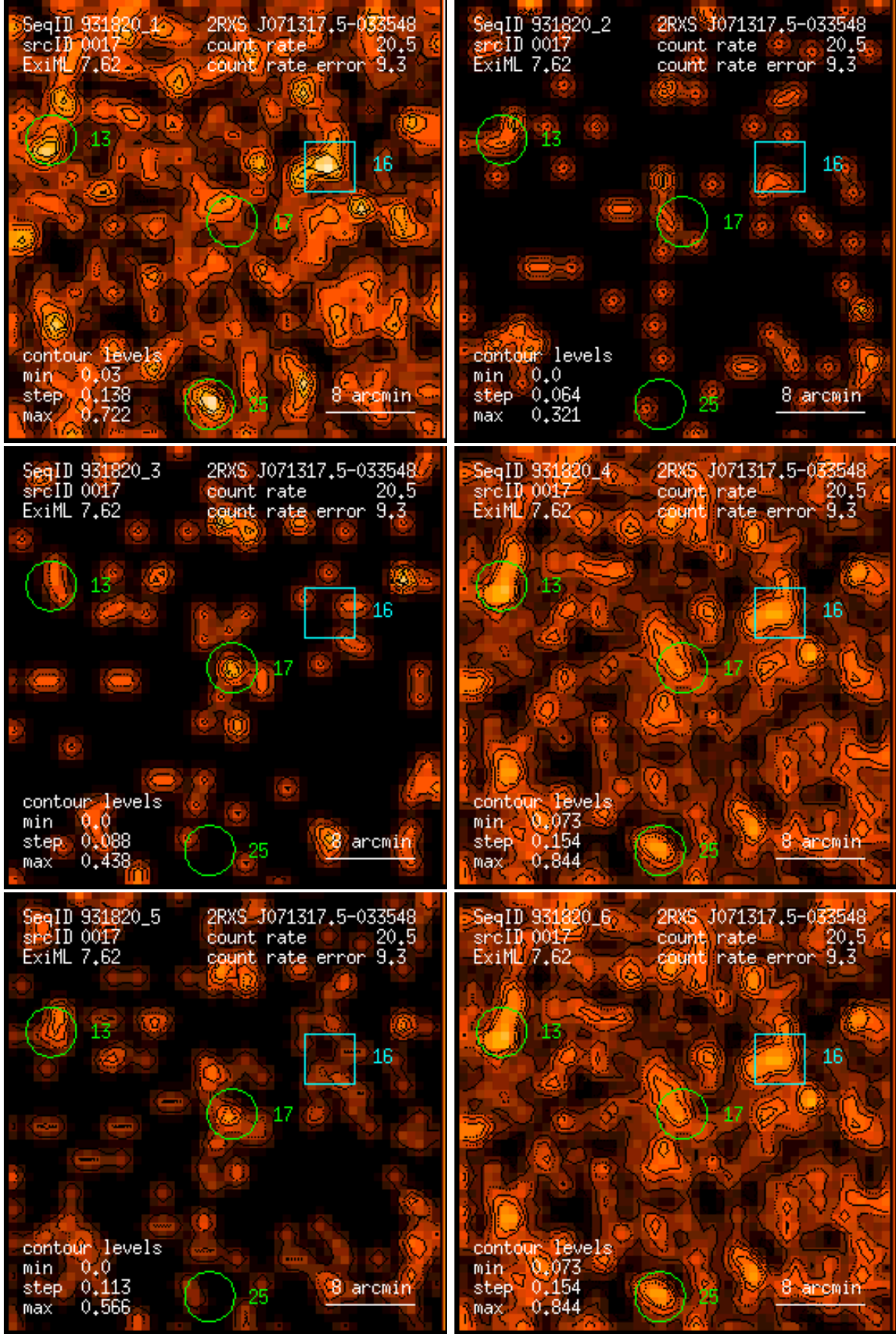
Figure 17: RASS 931820: detection 0017: band rate images, Gaussian filter: (1) PSPC channels 11 – 41, (2) 52 – 90, (3) 91 – 201, (4) 11 – 235, (5) 52 – 201, (6) 11 – 201. Broad band rates in counts/ks. Band rate contour levels in counts/ks/arcmin 2 .
