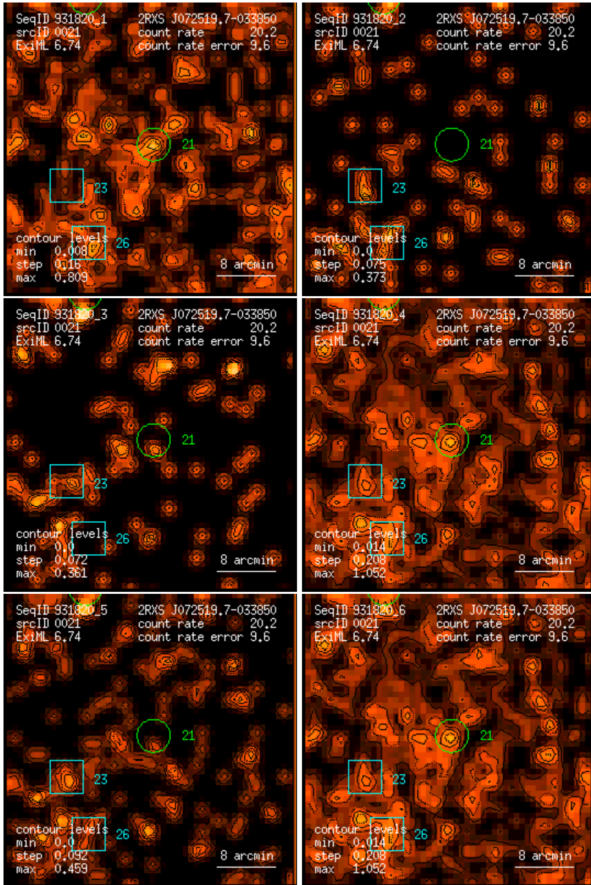
Figure 21: RASS 931820: detection 0021: band rate images, Gaussian filter: (1) PSPC channels 11 – 41, (2) 52 – 90, (3) 91 – 201, (4) 11 – 235, (5) 52 – 201, (6) 11 – 201. Broad band rates in counts/ks. Band rate contour levels in counts/ks/arcmin 2 .
