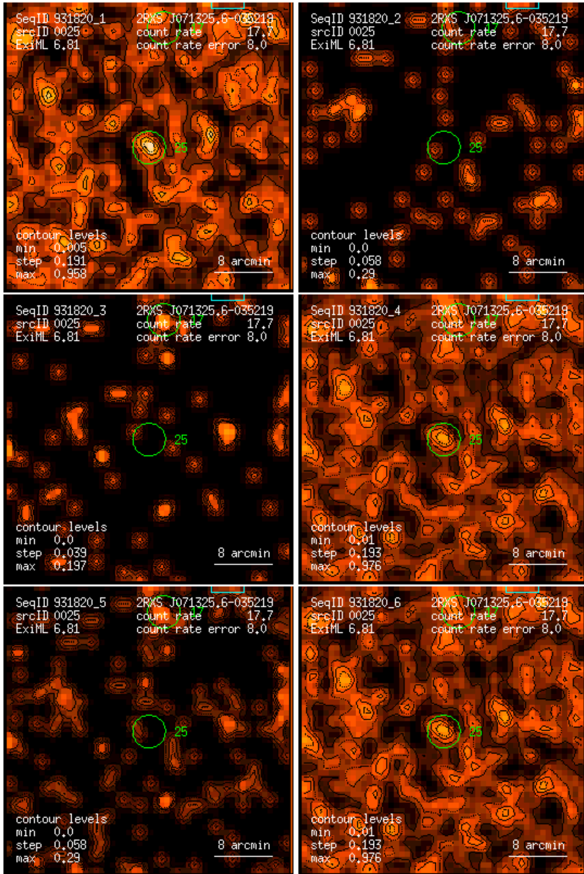
Figure 25: RASS 931820: detection 0025: band rate images, Gaussian filter: (1) PSPC channels 11 – 41, (2) 52 – 90, (3) 91 – 201, (4) 11 – 235, (5) 52 – 201, (6) 11 – 201. Broad band rates in counts/ks. Band rate contour levels in counts/ks/arcmin 2 .
