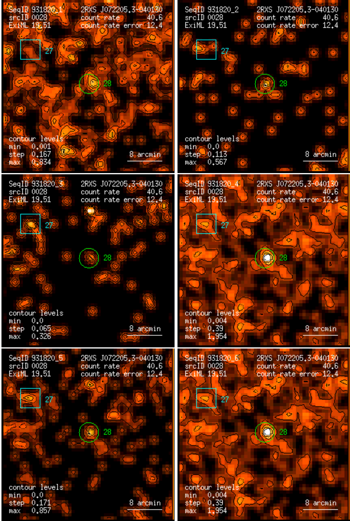
Figure 28: RASS 931820: detection 0028: band rate images, Gaussian filter: (1) PSPC channels 11 – 41, (2) 52 – 90, (3) 91 – 201, (4) 11 – 235, (5) 52 – 201, (6) 11 – 201. Broad band rates in counts/ks. Band rate contour levels in counts/ks/arcmin 2 .
