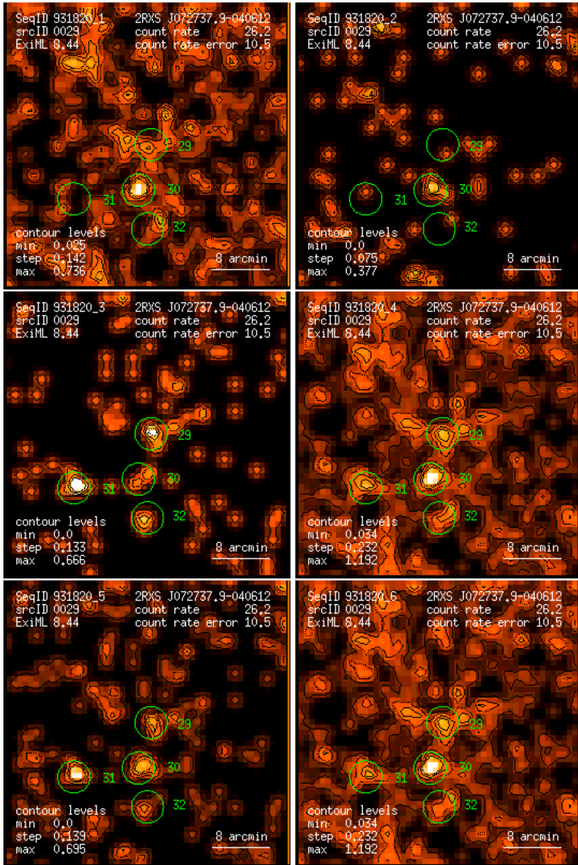
Figure 29: RASS 931820: detection 0029: band rate images, Gaussian filter: (1) PSPC channels 11 – 41, (2) 52 – 90, (3) 91 – 201, (4) 11 – 235, (5) 52 – 201, (6) 11 – 201. Broad band rates in counts/ks. Band rate contour levels in counts/ks/arcmin 2 .
