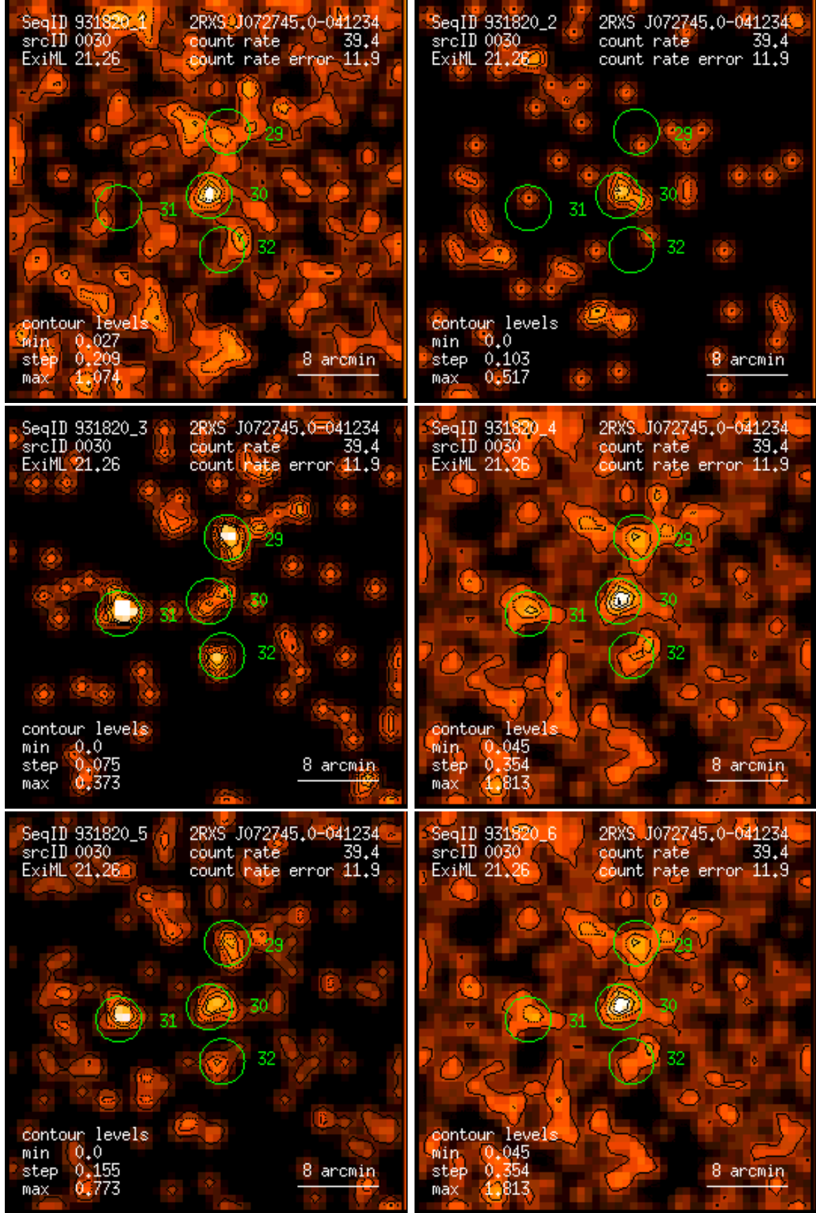
Figure 30: RASS 931820: detection 0030: band rate images, Gaussian filter: (1) PSPC channels 11 – 41, (2) 52 – 90, (3) 91 – 201, (4) 11 – 235, (5) 52 – 201, (6) 11 – 201. Broad band rates in counts/ks. Band rate contour levels in counts/ks/arcmin 2 .
