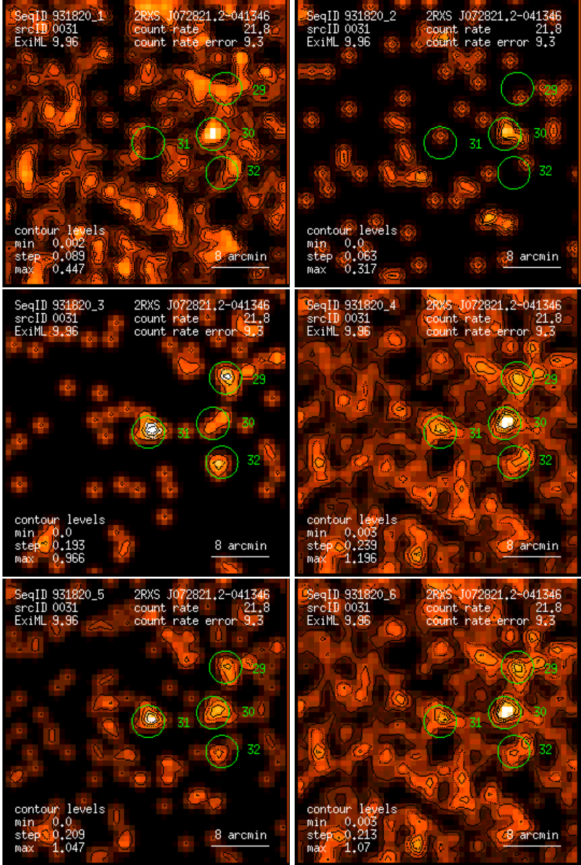
Figure 31: RASS 931820: detection 0031: band rate images, Gaussian filter: (1) PSPP channels 11 – 41, (2) 52 – 90, (3) 91 – 201, (4) 11 – 235, (5) 52 – 201, (6) 11 – 201. Broad band rates in counts/ks. Band rate contour levels in counts/ks/arcmin 2 .
