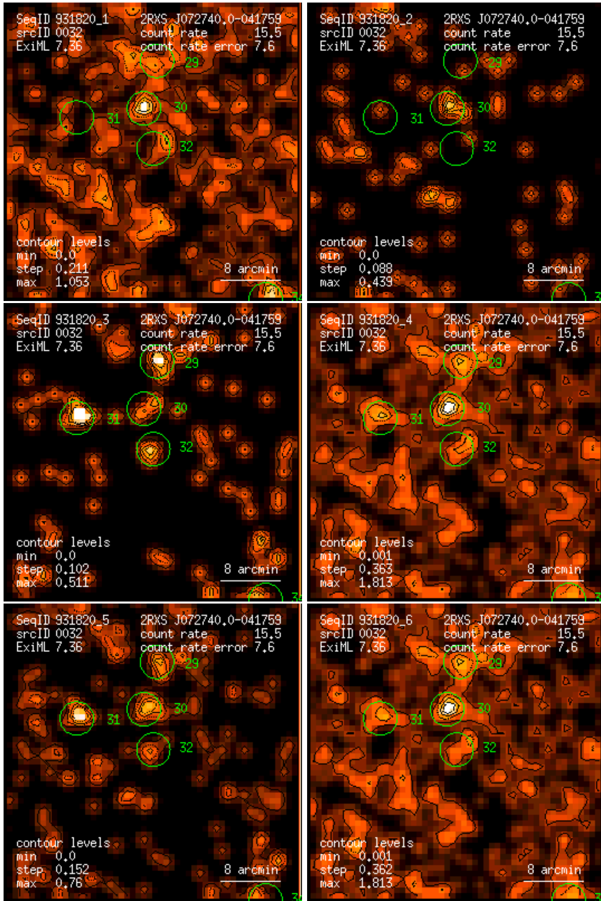
Figure 32: RASS 931820: detection 0032: band rate images, Gaussian filter: (1) PSPC channels 11 – 41, (2) 52 – 90, (3) 91 – 201, (4) 11 – 235, (5) 52 – 201, (6) 11 – 201. Broad band rates in counts/ks. Band rate contour levels in counts/ks/arcmin 2 .
