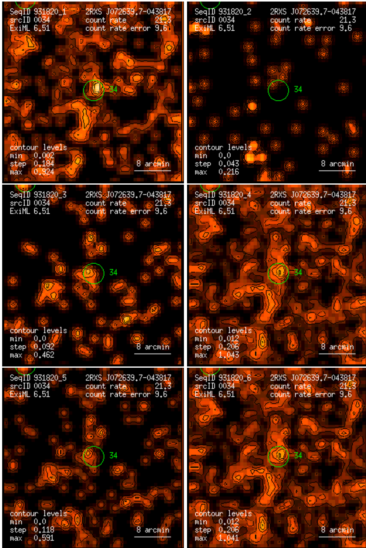
Figure 34: RASS 931820: detection 0034: band rate images, Gaussian filter: (1) PSPC channels 11 – 41, (2) 52 – 90, (3) 91 – 201, (4) 11 – 235, (5) 52 – 201, (6) 11 – 201. Broad band rates in counts/ks. Band rate contour levels in counts/ks/arcmin 2 .
