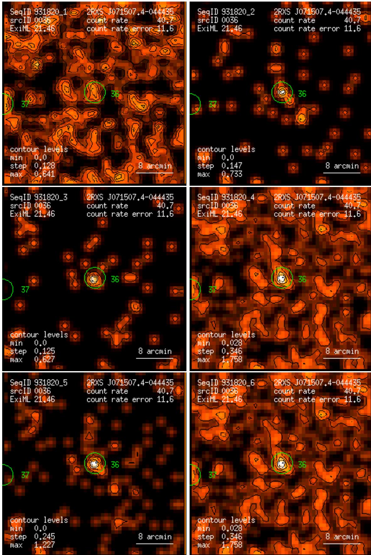
Figure 36: RASS 931820: detection 0036: band rate images, Gaussian filter: (1) PSPC channels 11 – 41, (2) 52 – 90, (3) 91 – 201, (4) 11 – 235, (5) 52 – 201, (6) 11 – 201. Broad band rates in counts/ks. Band rate contour levels in counts/ks/arcmin 2 .
