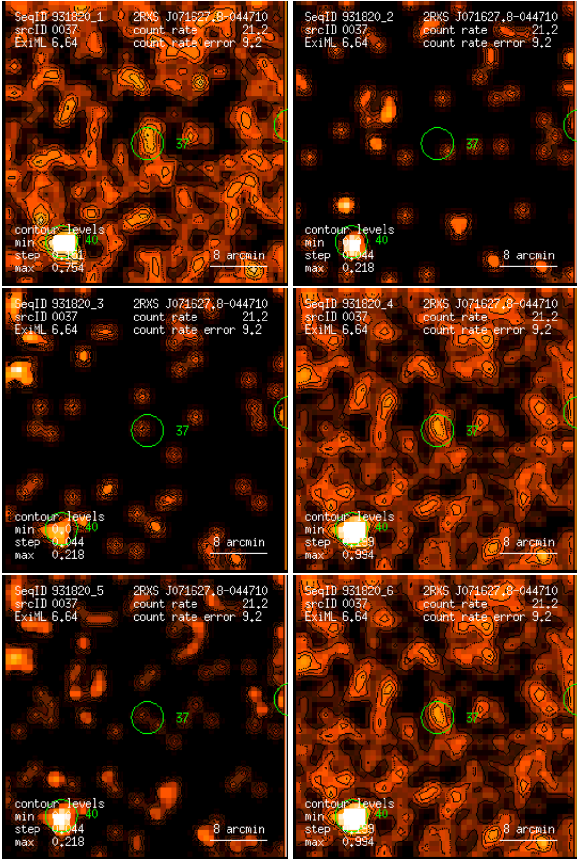
Figure 37: RASS 931820: detection 0037: band rate images, Gaussian filter: (1) PSPC channels 11 – 41, (2) 52 – 90, (3) 91 – 201, (4) 11 – 235, (5) 52 – 201, (6) 11 – 201. Broad band rates in counts/ks. Band rate contour levels in counts/ks/arcmin 2 .
