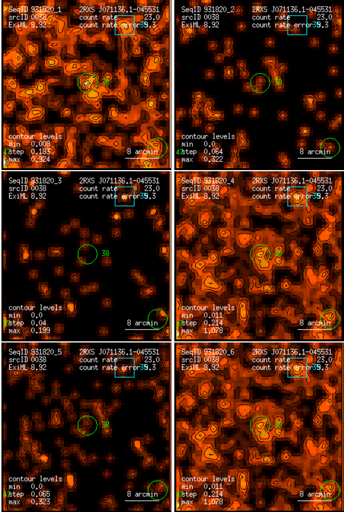
Figure 38: RASS 931820: detection 0038: band rate images, Gaussian filter: (1) PSPC channels 11 – 41, (2) 52 – 90, (3) 91 – 201, (4) 11 – 235, (5) 52 – 201, (6) 11 – 201. Broad band rates in counts/ks. Band rate contour levels in counts/ks/arcmin 2 .
