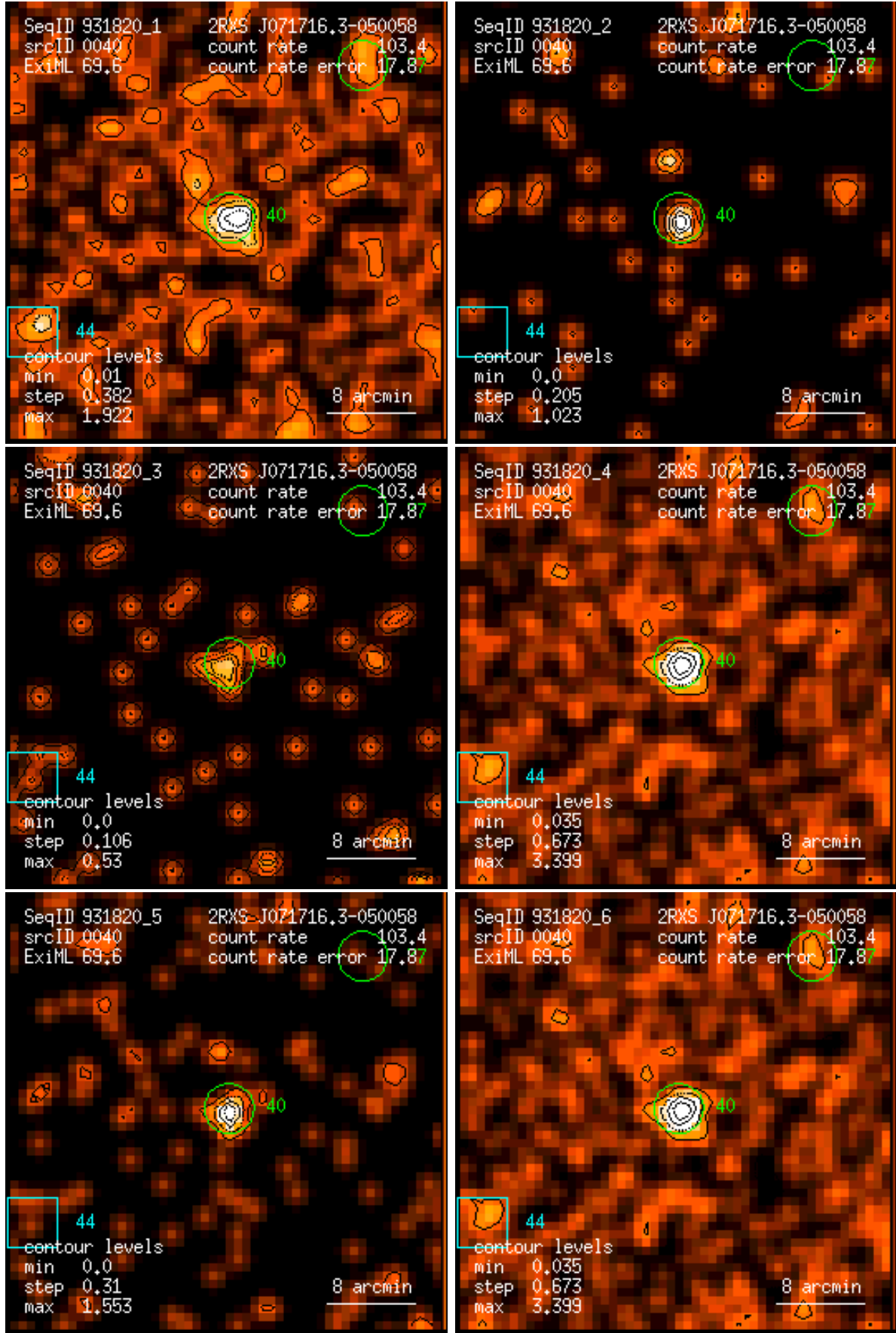
Figure 40: RASS 931820: detection 0040: band rate images, Gaussian filter: (1) PSPC channels 11 – 41, (2) 52 – 90, (3) 91 – 201, (4) 11 – 235, (5) 52 – 201, (6) 11 – 201. Broad band rates in counts/ks. Band rate contour levels in counts/ks/arcmin 2 .
