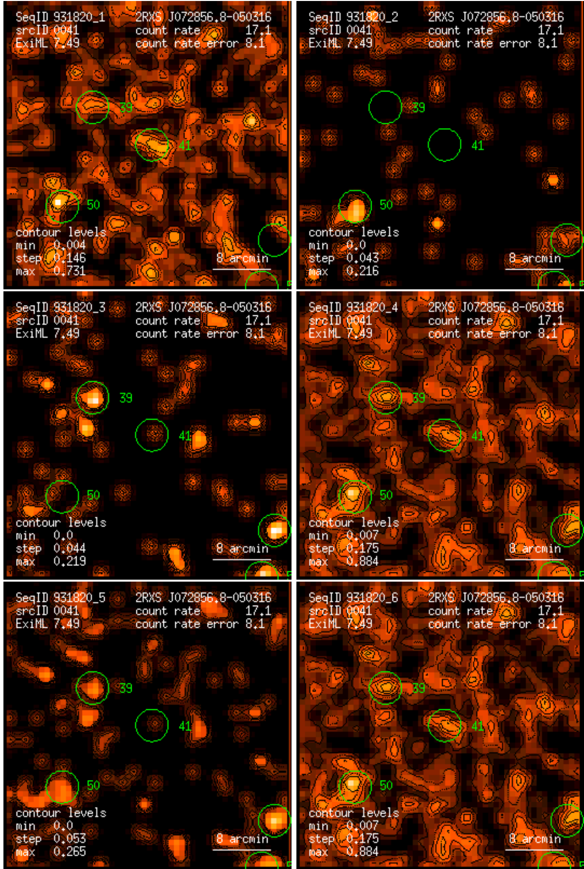
Figure 41: RASS 931820: detection 0041: band rate images, Gaussian filter: (1) PSPC channels 11 – 41, (2) 52 – 90, (3) 91 – 201, (4) 11 – 235, (5) 52 – 201, (6) 11 – 201. Broad band rates in counts/ks. Band rate contour levels in counts/ks/arcmin 2 .
