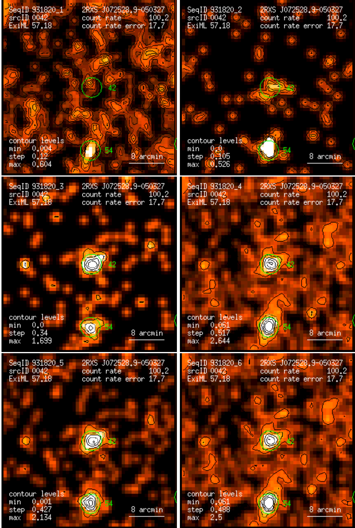
Figure 42: RASS 931820: detection 0042: band rate images, Gaussian filter: (1) PSPC channels 11 – 41, (2) 52 – 90, (3) 91 – 201, (4) 11 – 235, (5) 52 – 201, (6) 11 – 201. Broad band rates in counts/ks. Band rate contour levels in counts/ks/arcmin 2 .
