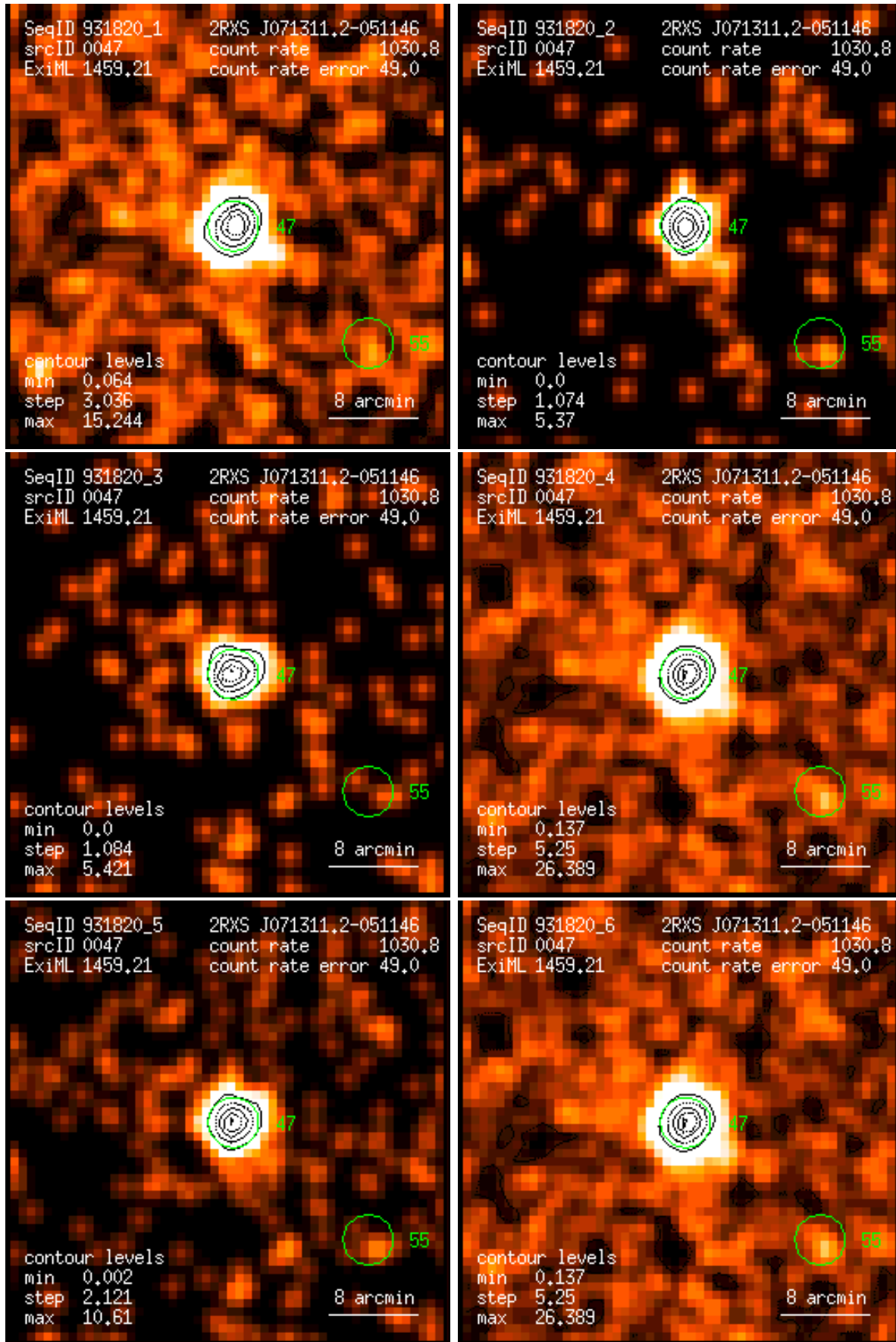
Figure 47: RASS 931820: detection 0047: band rate images, Gaussian filter: (1) PSPC channels 11 – 41, (2) 52 – 90, (3) 91 – 201, (4) 11 – 235, (5) 52 – 201, (6) 11 – 201. Broad band rates in counts/ks. Band rate contour levels in counts/ks/arcmin 2 .
