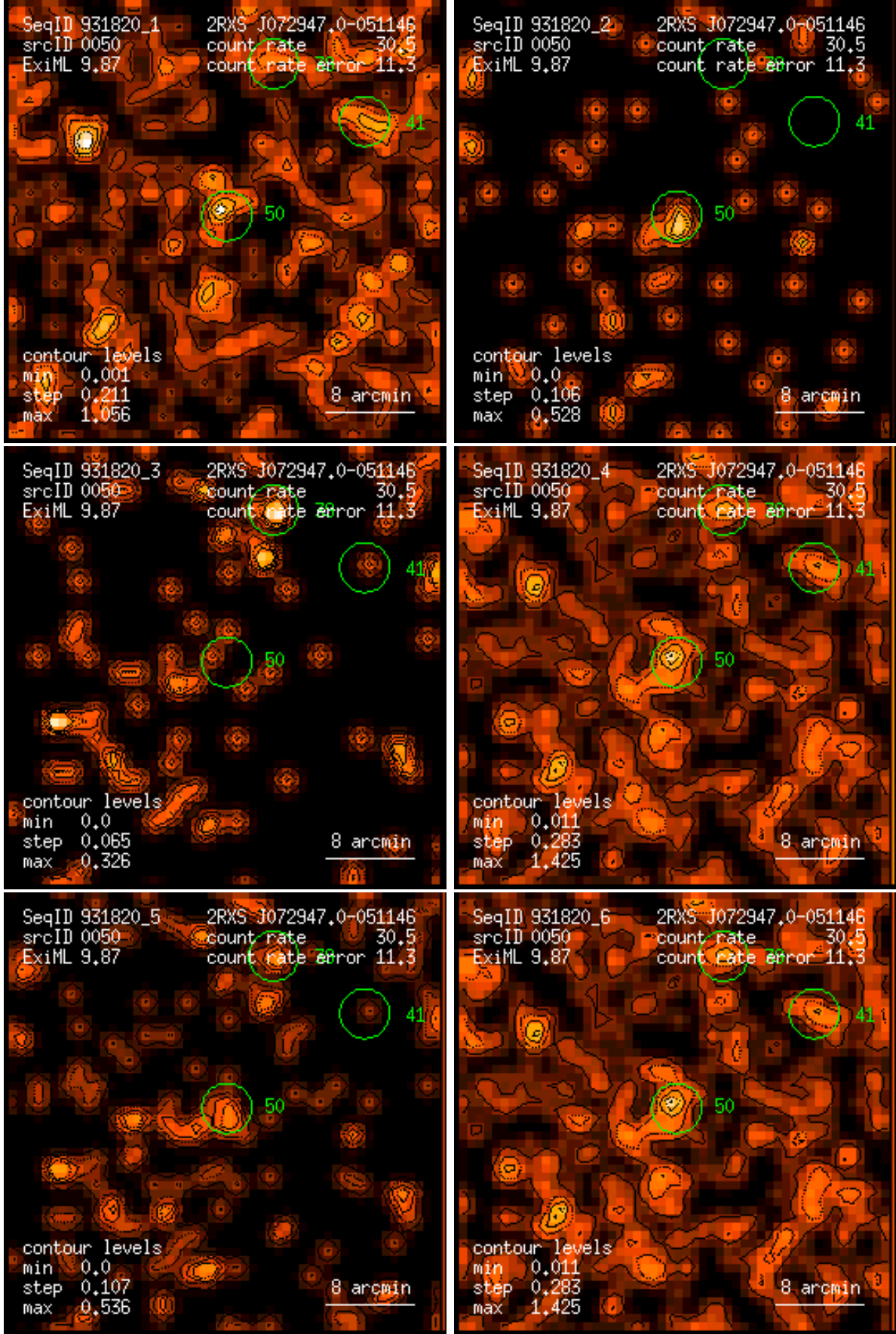
Figure 50: RASS 931820: detection 0050: band rate images, Gaussian filter: (1) PSPC channels 11 – 41, (2) 52 – 90, (3) 91 – 201, (4) 11 – 235, (5) 52 – 201, (6) 11 – 201. Broad band rates in counts/ks. Band rate contour levels in counts/ks/arcmin 2 .
