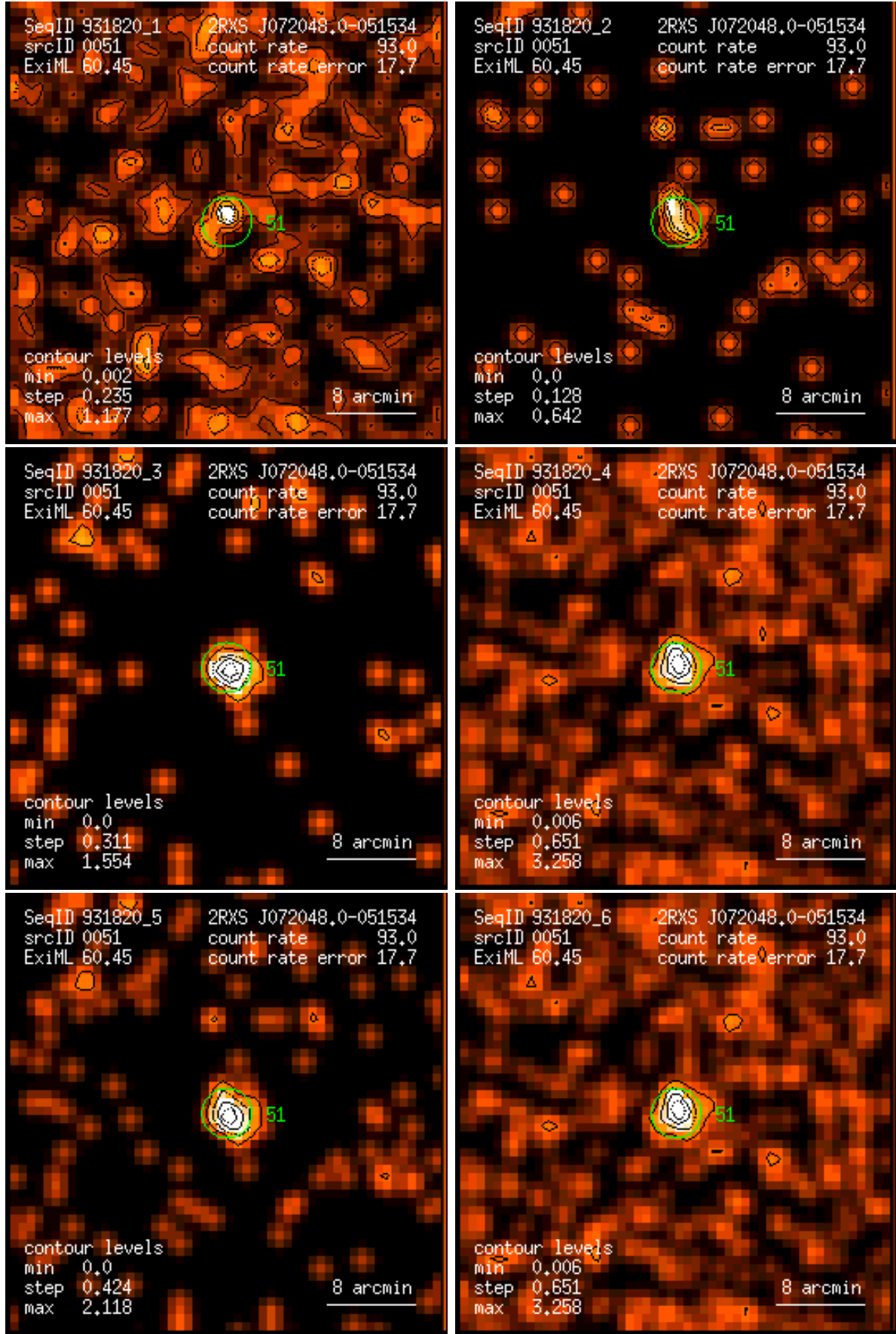
Figure 51: RASS 931820: detection 0051: band rate images, Gaussian filter: (1) PSPC channels 11 – 41, (2) 52 – 90, (3) 91 – 201, (4) 11 – 235, (5) 52 – 201, (6) 11 – 201. Broad band rates in counts/ks. Band rate contour levels in counts/ks/arcmin 2 .
