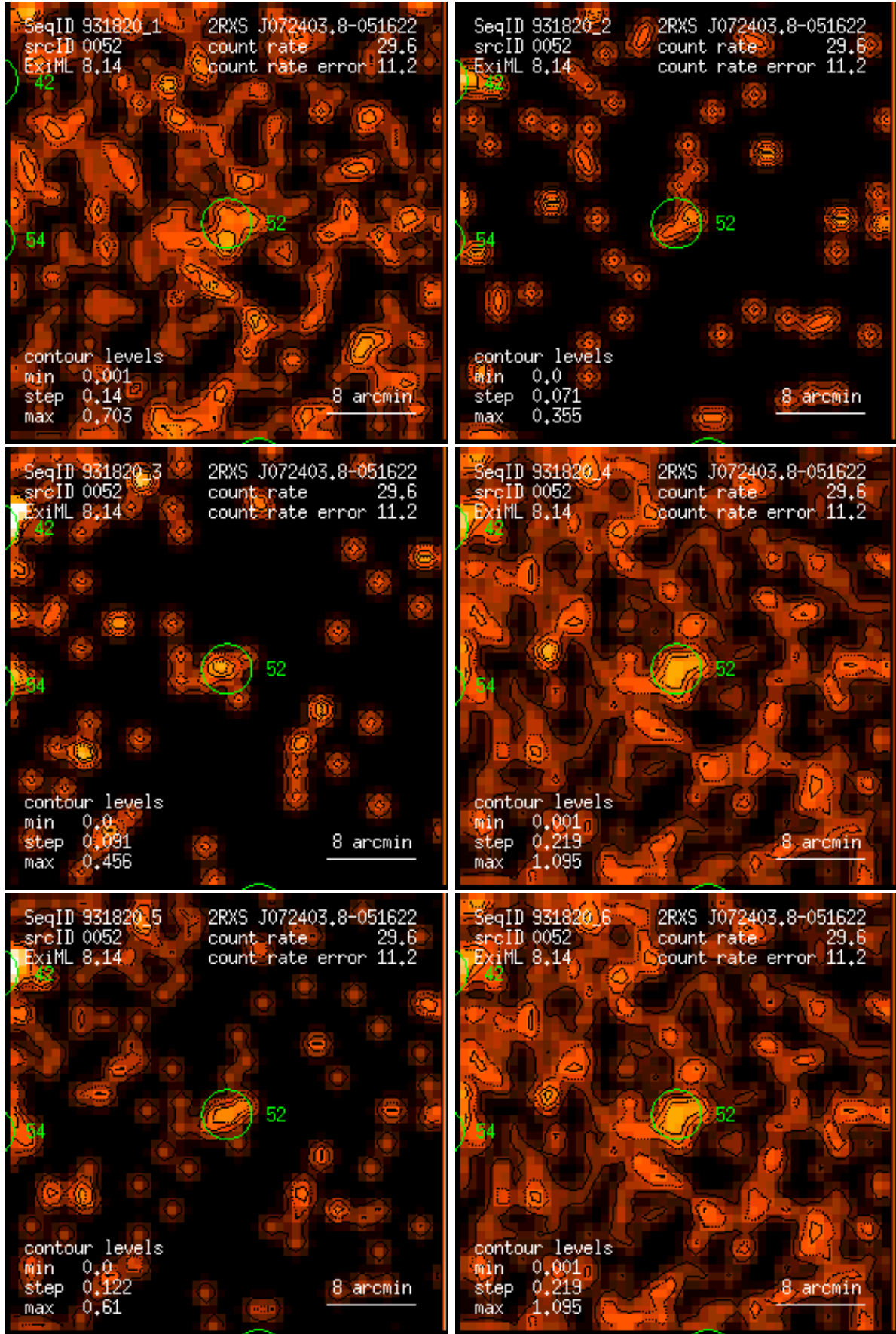
Figure 52: RASS 931820: detection 0052: band rate images, Gaussian filter: (1) PSPP channels 11 – 41, (2) 52 – 90, (3) 91 – 201, (4) 11 – 235, (5) 52 – 201, (6) 11 – 201. Broad band rates in counts/ks. Band rate contour levels in counts/ks/arcmin 2 .
