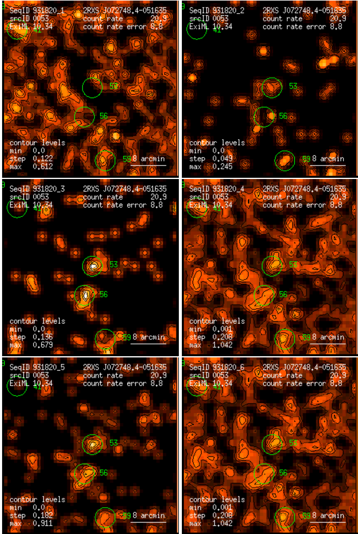
Figure 53: RASS 931820: detection 0053: band rate images, Gaussian filter: (1) PSPC channels 11 – 41, (2) 52 – 90, (3) 91 – 201, (4) 11 – 235, (5) 52 – 201, (6) 11 – 201. Broad band rates in counts/ks. Band rate contour levels in counts/ks/arcmin 2 .
