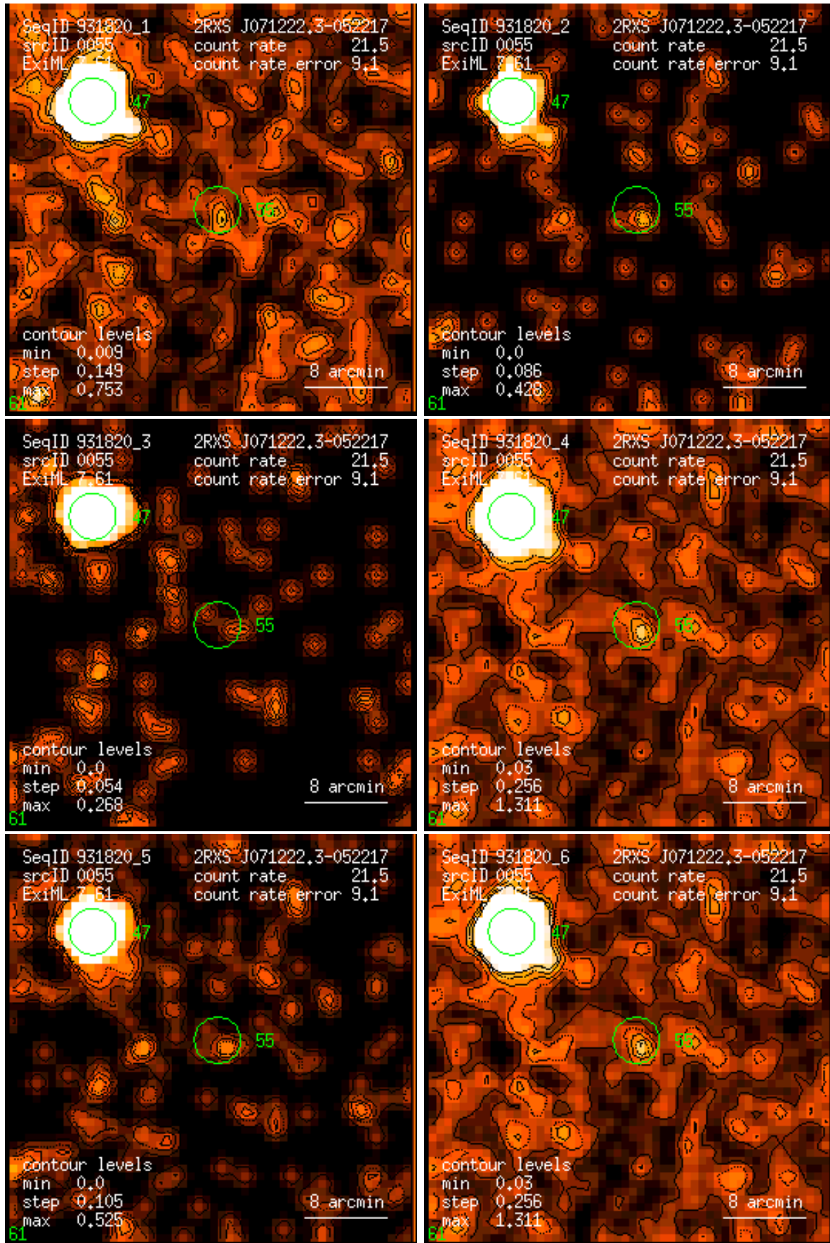
Figure 55: RASS 931820: detection 0055: band rate images, Gaussian filter: (1) PSPC channels 11 – 41, (2) 52 – 90, (3) 91 – 201, (4) 11 – 235, (5) 52 – 201, (6) 11 – 201. Broad band rates in counts/ks. Band rate contour levels in counts/ks/arcmin 2 .
