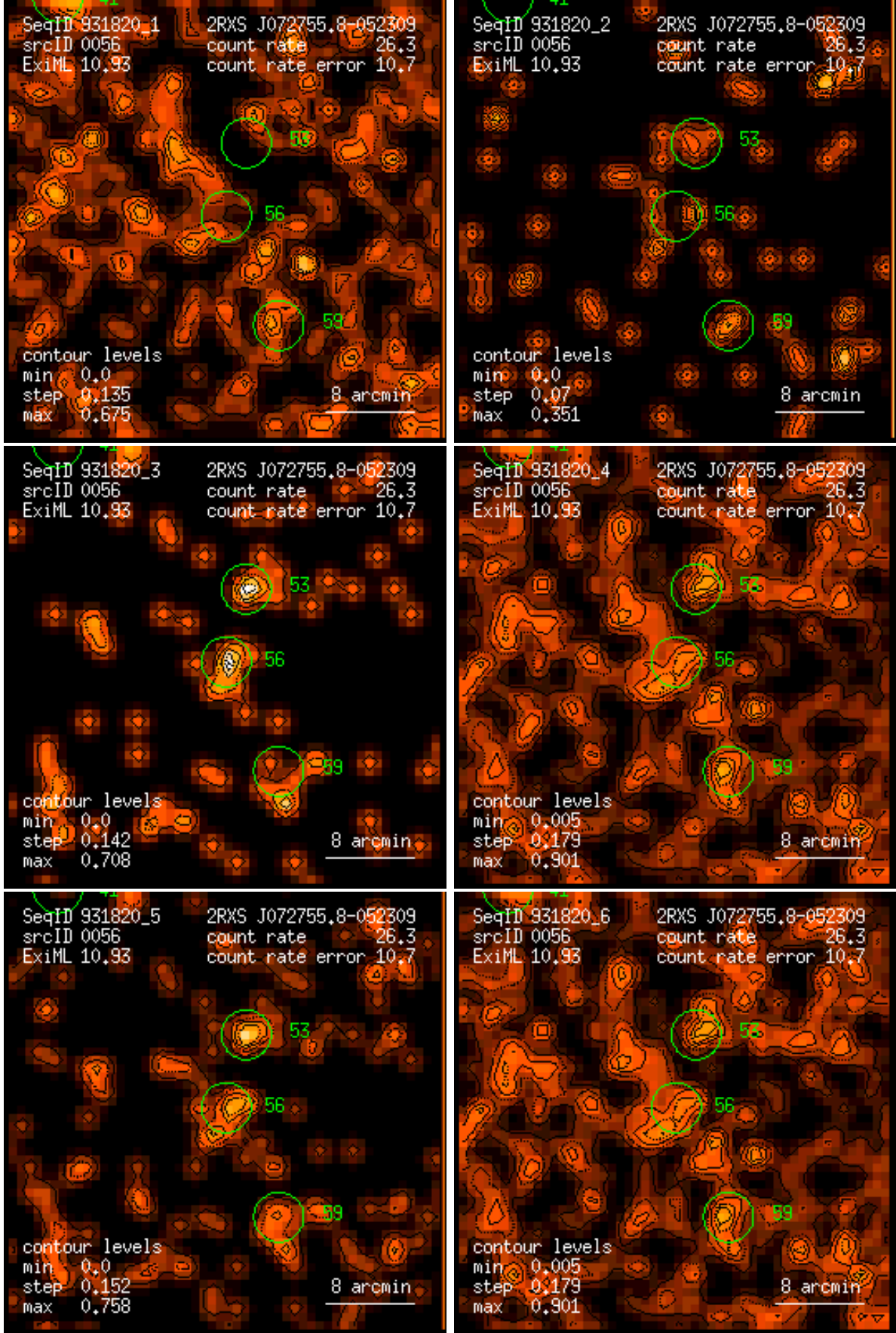
Figure 56: RASS 931820: detection 0056: band rate images, Gaussian filter: (1) PSPC channels 11 – 41, (2) 52 – 90, (3) 91 – 201, (4) 11 – 235, (5) 52 – 201, (6) 11 – 201. Broad band rates in counts/ks. Band rate contour levels in counts/ks/arcmin 2 .
