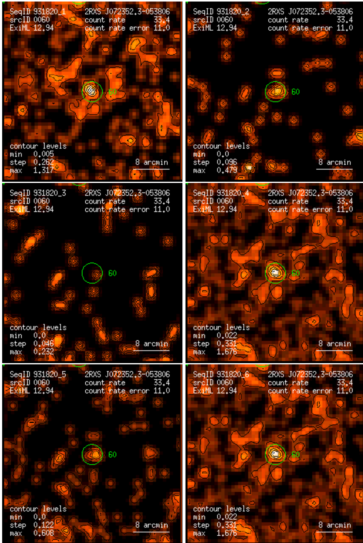
Figure 60: RASS 931820: detection 0060: band rate images, Gaussian filter: (1) PSPC channels 11 – 41, (2) 52 – 90, (3) 91 – 201, (4) 11 – 235, (5) 52 – 201, (6) 11 – 201. Broad band rates in counts/ks. Band rate contour levels in counts/ks/arcmin 2 .
