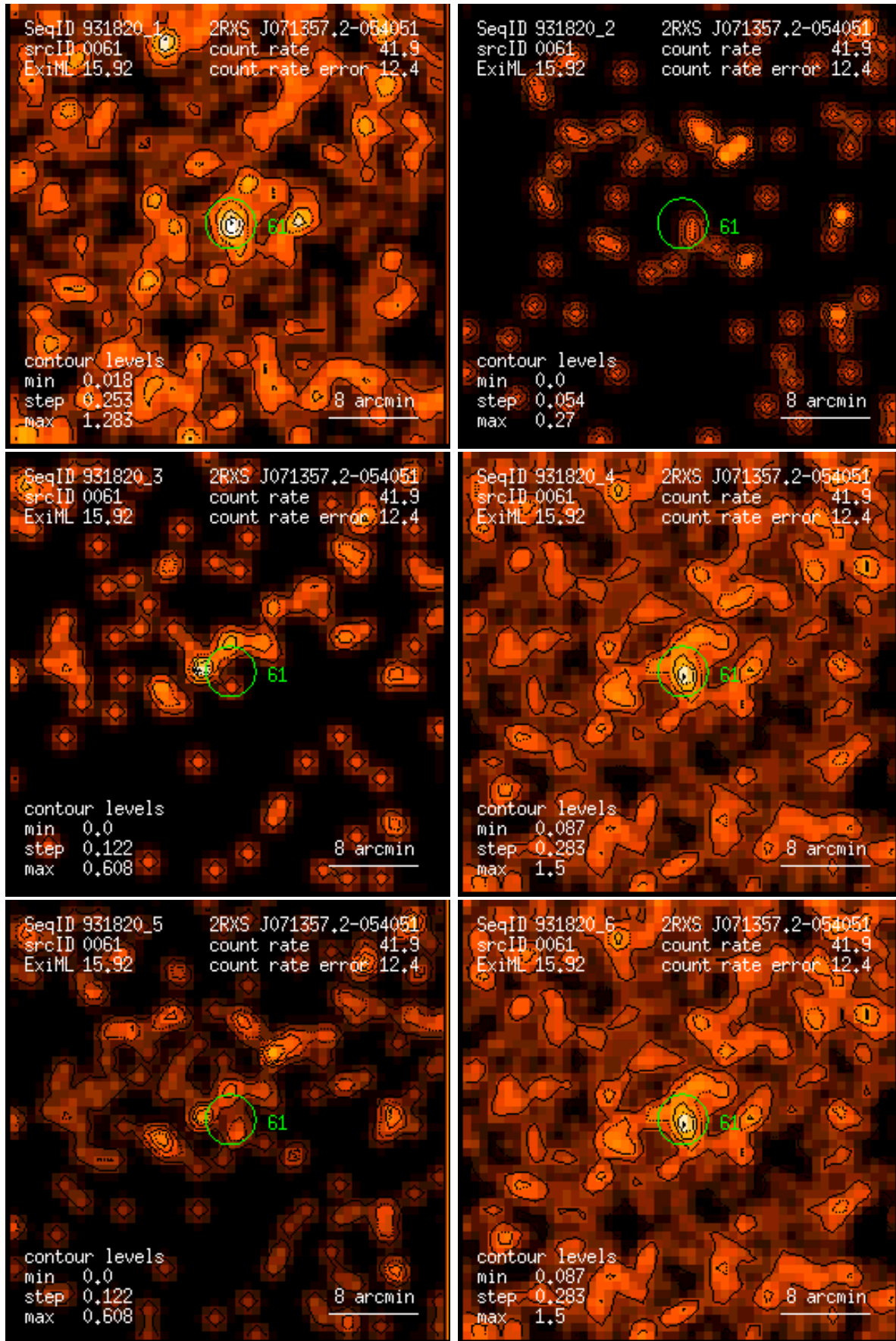
Figure 61: RASS 931820: detection 0061: band rate images, Gaussian filter: (1) PSPC channels 11 – 41, (2) 52 – 90, (3) 91 – 201, (4) 11 – 235, (5) 52 – 201, (6) 11 – 201. Broad band rates in counts/ks. Band rate contour levels in counts/ks/arcmin 2 .
