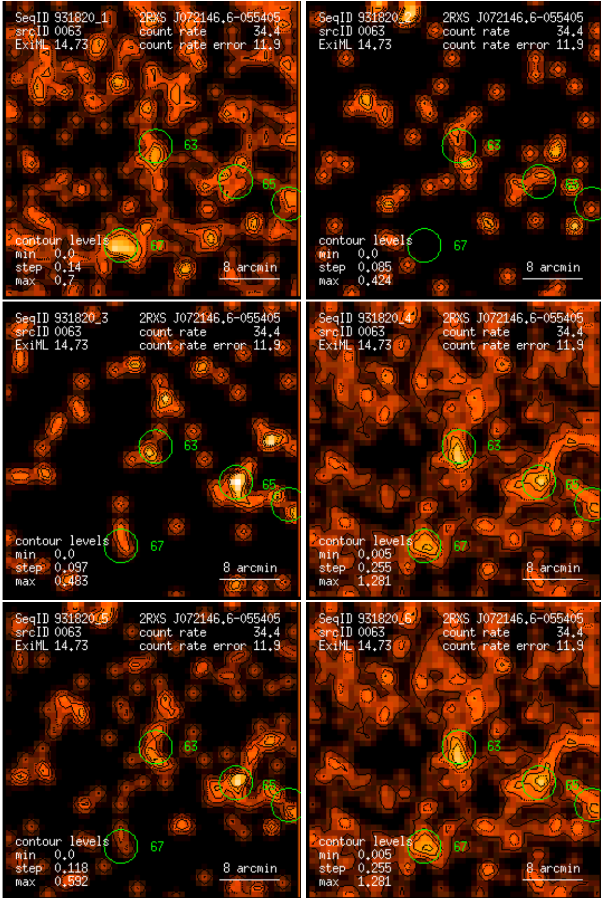
Figure 63: RASS 931820: detection 0063: band rate images, Gaussian filter: (1) PSPC channels 11 – 41, (2) 52 – 90, (3) 91 – 201, (4) 11 – 235, (5) 52 – 201, (6) 11 – 201. Broad band rates in counts/ks. Band rate contour levels in counts/ks/arcmin 2 .
