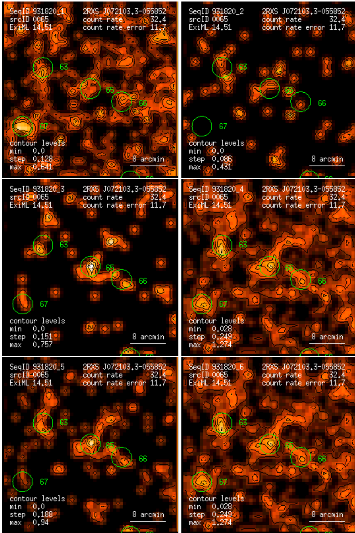
Figure 65: RASS 931820: detection 0065: band rate images, Gaussian filter: (1) PSPC channels 11 – 41, (2) 52 – 90, (3) 91 – 201, (4) 11 – 235, (5) 52 – 201, (6) 11 – 201. Broad band rates in counts/ks. Band rate contour levels in counts/ks/arcmin 2 .
