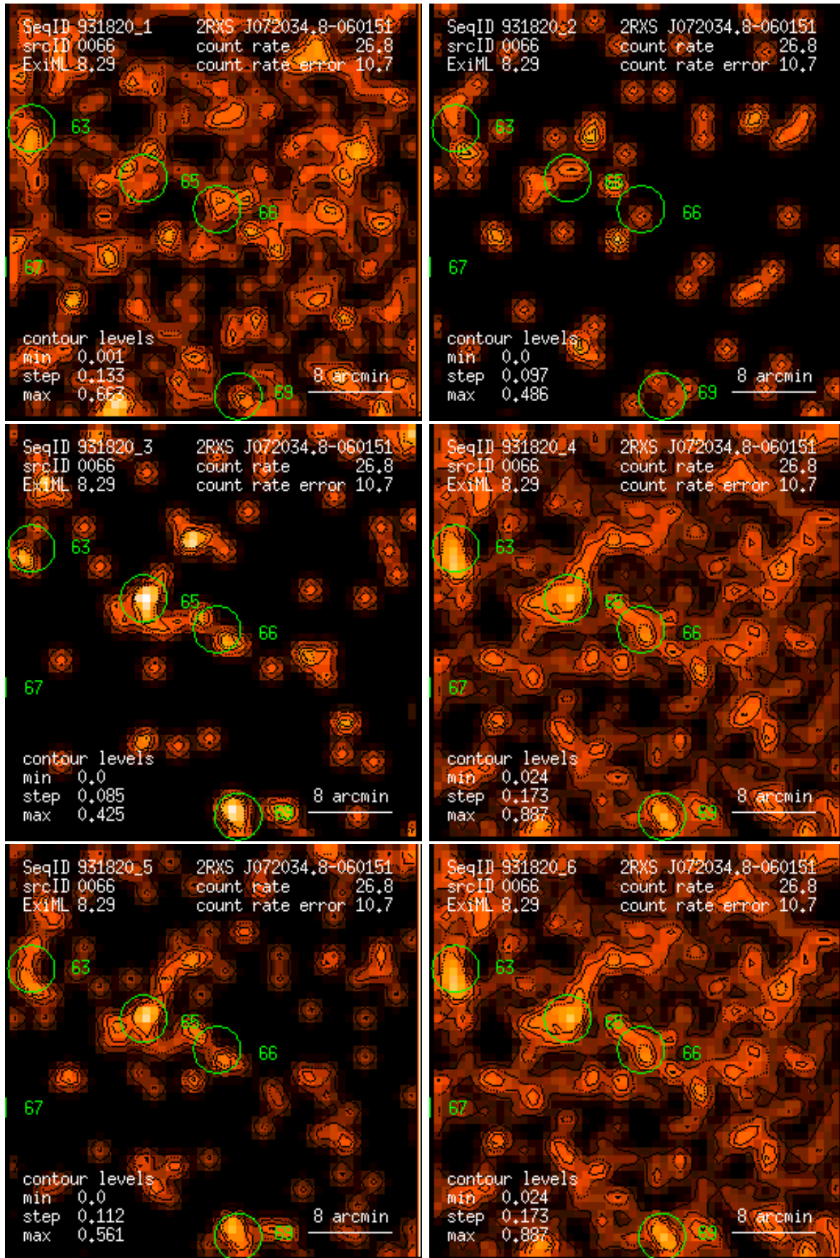
Figure 66: RASS 931820: detection 0066: band rate images, Gaussian filter: (1) PSPC channels 11 – 41, (2) 52 – 90, (3) 91 – 201, (4) 11 – 235, (5) 52 – 201, (6) 11 – 201. Broad band rates in counts/ks. Band rate contour levels in counts/ks/arcmin 2 .
