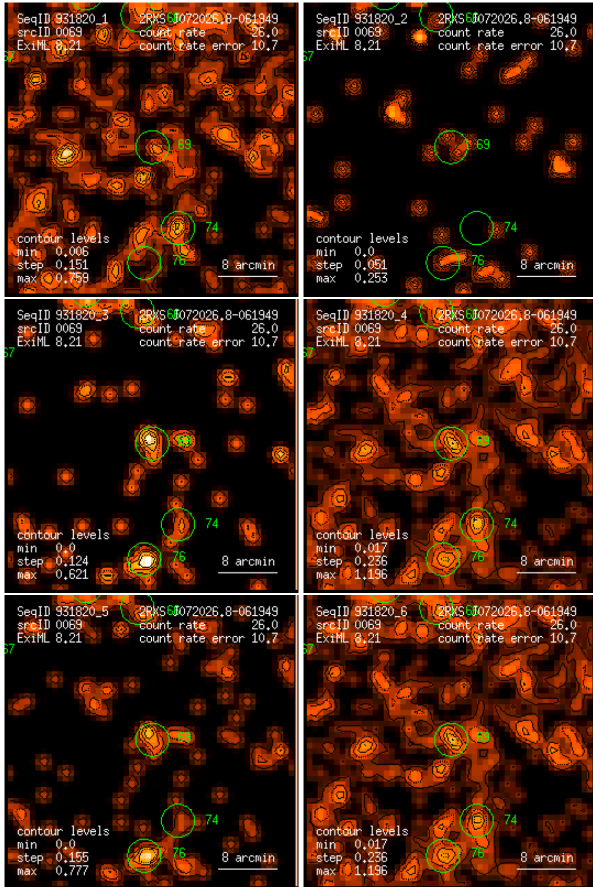
Figure 69: RASS 931820: detection 0069: band rate images, Gaussian filter: (1) PSPC channels 11 – 41, (2) 52 – 90, (3) 91 – 201, (4) 11 – 235, (5) 52 – 201, (6) 11 – 201. Broad band rates in counts/ks. Band rate contour levels in counts/ks/arcmin 2 .
