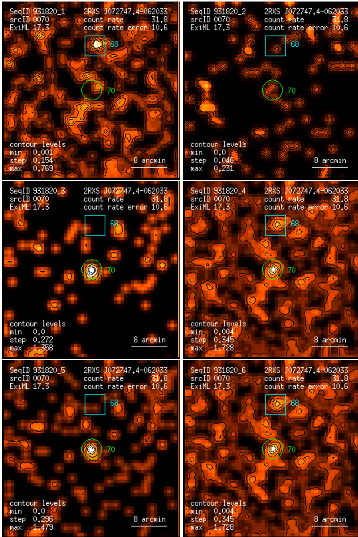
Figure 70: RASS 931820: detection 0070: band rate images, Gaussian filter: (1) PSPC channels 11 – 41, (2) 52 – 90, (3) 91 – 201, (4) 11 – 235, (5) 52 – 201, (6) 11 – 201. Broad band rates in counts/ks. Band rate contour levels in counts/ks/arcmin 2 .
